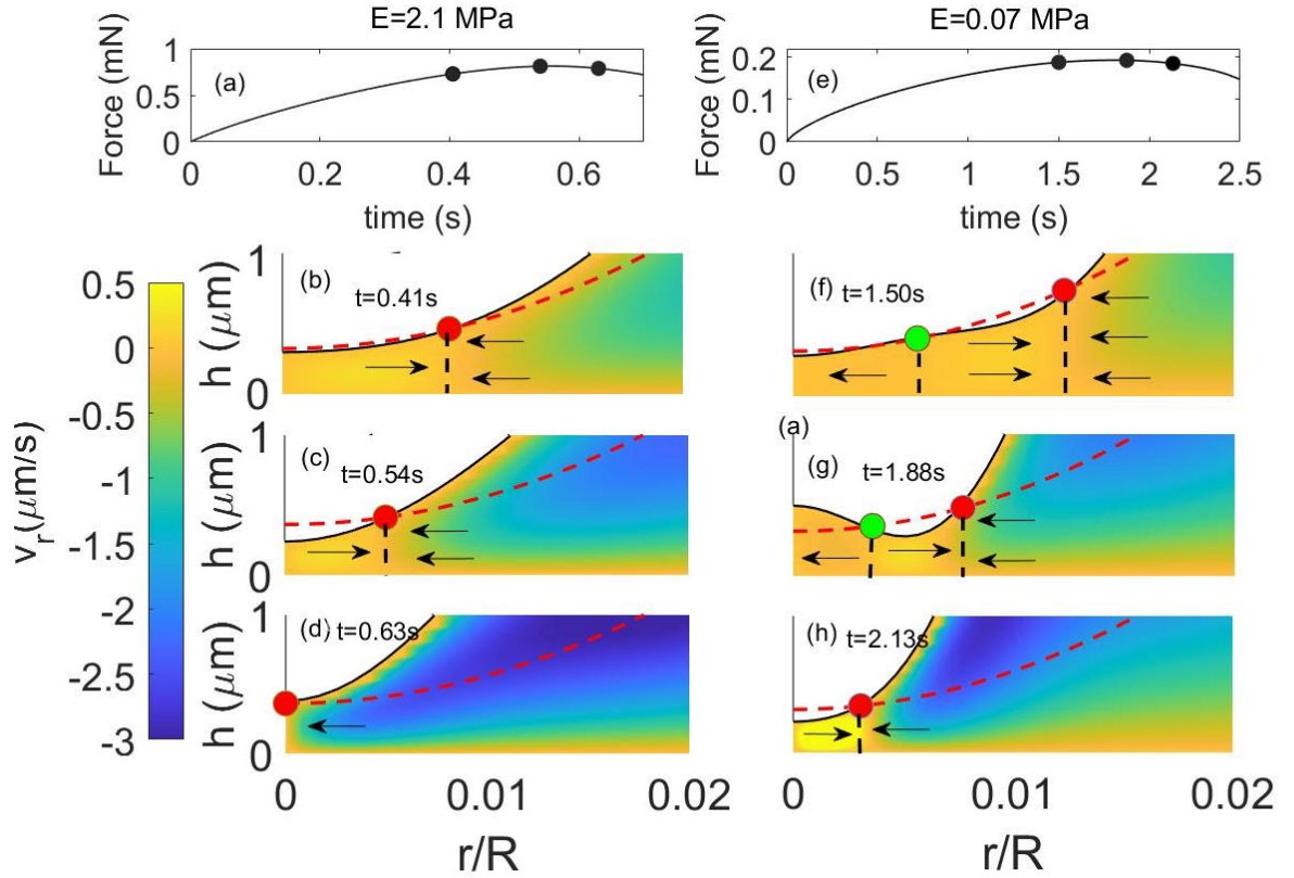
Fig. 7. Velocity field contour in temporal sequence during retraction at V = 3.5 \mu\text{m/s} with \eta = 0.22 \text{ Pa} \cdot \text{s} , h_0 = 300 \text{ nm} for (a-d) E = 2.10 \text{ MPa} with the time points shown in the force curve in (a), and (e-h) E = 0.07 \text{ MPa} , with the time points shown in the force curve in (e). The red dashed lines represent the initial (underformed) fluid film thickness h(r, t = 0) . The colored points represent the locations of the stagnation points. We observe one stagnation point (red) at E = 2.1 \text{ MPa} , whereas two stagnation points (red
