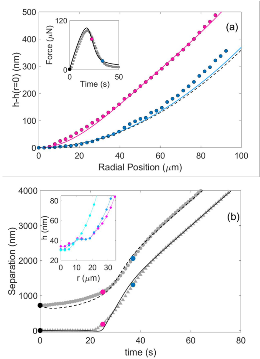
Figure 3. (a) Direct measurement of fluid film thickness during retraction using the SFA showing the out-of-contact peeling process. Solid lines represent model prediction without any adjustable parameters, but with a shifted hydrodynamic plane of 35 nm due to surface roughness. 11 Experimental conditions are V = 61 \mu\text{m/s} , \eta = 0.194 \text{ Pa} \cdot \text{s} , h_0 = 35 \text{ nm} , E = 1.05 \text{ MPa} and R = 13.1 \text{ mm} . Black dashed lines represent the initial film thickness profile. Inset: force versus time data during retraction process along with model prediction. Colored data points represent data taken at the same time. The pink points and line are taken at a time with the largest central deformation. (b) Experiments and model prediction for the temporal film thickness at the centerpoint (triangles, solid line) and at \frac{r}{R} = 0.01 (circles, dash line). The colored points serve as indicators for the force curve shown in the inset in (a) and the inset shows the surface profile
