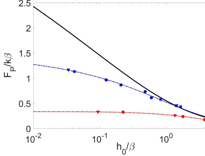
Fig. 4. Model predictions of the peak force ( F_p ) against scaled initial separation for the detachment from an elastic substrate with E = 2.1 MPa (dashed blue line) and E = 0.07 MPa (dashed red line) respectively, at V=3.5, 7 , and 10 \frac{\mu\text{m}}{\text{s}} and fluid viscosity \eta = 2.2 , and 5.3 \text{ Pa} \cdot \text{s} . The characteristic length \beta = [\frac{6\pi\eta R^2 V}{k_{spring}}]^{1/2} represents the balance between spring force and viscous force. The cantilever spring constant k = k_{spring} is used in the nondimensionalization. The data collapses on a single curve for the different experimental parameters but the curves do not collapse for different Young's moduli. The relationship for the viscous adhesion between rigid surfaces (solid black line) is from Horn et. al. 25 and is used as a benchmark for the case of F_p where no elastic deformation is present. The blue points represent the experimental data for E = 2.1 MPa at V = 3.5 \frac{\mu\text{m}}{\text{s}}, \eta = 2.2 \text{ Pa} \cdot \text{s} (square); V = 7 \frac{\mu\text{m}}{\text{s}}, \eta = 2.2 \text{ Pa} \cdot \text{s} (circle); V = 10 \frac{\mu\text{m}}{\text{s}}, \eta = 5.3 \text{ Pa} \cdot \text{s} (triangle). The red points represents the result of E = 0.07 MPa at V = 3.5 \frac{\mu\text{m}}{\text{s}}, \eta = 5.3 \text{ Pa} \cdot \text{s} (triangle); and V = 10 \frac{\mu\text{m}}{\text{s}}, \eta = 5.3 \text{ Pa} \cdot \text{s} (circles).
