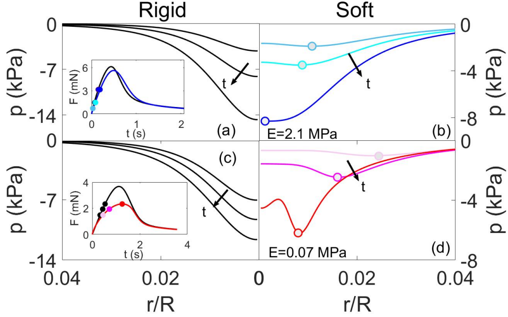
Fig. 6. Role of surface compliance on pressure distribution. Pressure distribution during retraction calculated at different time points with V = 10 \mu\text{m/s} , \eta = 0.53 \text{ Pa}\cdot\text{s} , and h_0 = 900 \text{ nm} . (a) rigid surface (black curves) with the same effective stiffness as (b) E = 2.1 \text{ MPa} (blue curves). (c) rigid surface (black curves) with the same effective stiffness as (d) E = 0.07 \text{ MPa} (red curves). Inset of (a) and (c) shows the corresponding force curve where the detachment force for the rigid surface is in black and the soft surface is the colored line. Time progression is indicated with arrows as well as with lighter colored lines. The time points selected are shown in the force curves in the inset. The stagnation points are indicated by the highlighted points in (b), and (c).
