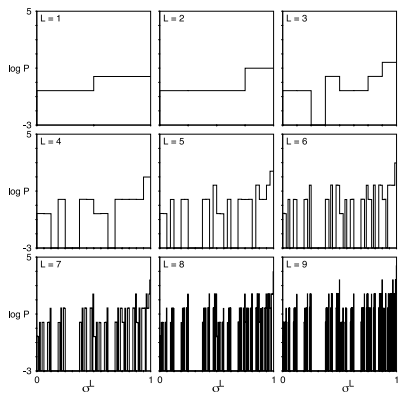
FIG. 2: Even Process stochastic language: Words \{01^{2k-1}0\} , k = 1, 2, 3, \dots have zero probability; all others have nonzero probability. The logarithm base 2 of the word probabilities is plotted versus the binary string s^L , represented as base-2 real number “ 0.s^L ”. To allow word probabilities to be compared at different lengths, the distribution is normalized on [0, 1] —that is, the probabilities are calculated as densities.
