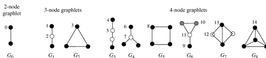
Figure 2. 2–4-node graphlets G_0 – G_8 and their automorphism orbits0–orbits14 [25].
