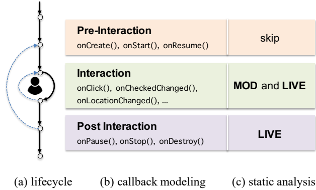
Figure 4.2: Callback Modeling and Static Analysis.
