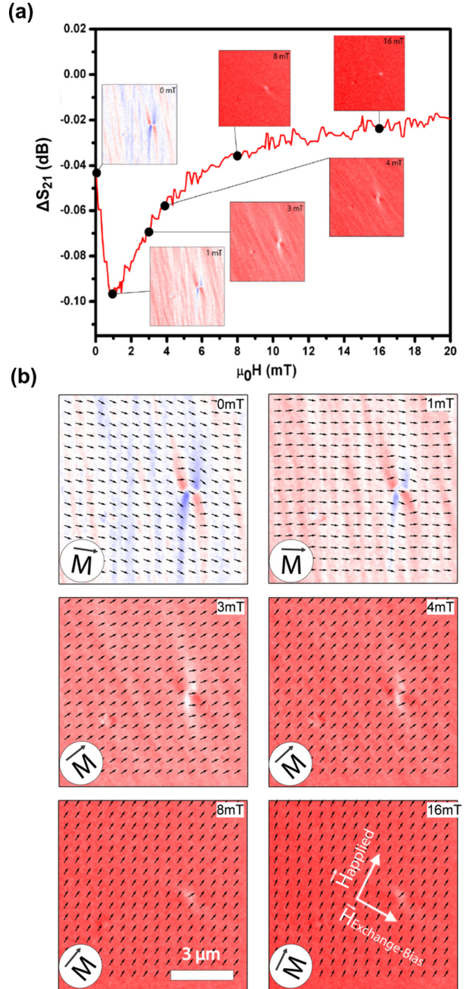
FIG. 3. (a) SAW damping \Delta S_{21} versus applied magnetic field together with XMCD-PEEM images (b) of the field-dependent magnetic state of CoFeB illustrate the magnetic domains. The circles in the lower left corner of each image represents the orientation of the net magnetization in the CoFeB thin film. Red color marks the fully aligned ferromagnetic layer along the external field, while blue color indicates a local deviation of magnetic spins in zero field and the matrix of arrows maps the local direction of magnetization at the surface of the ferromagnet.
