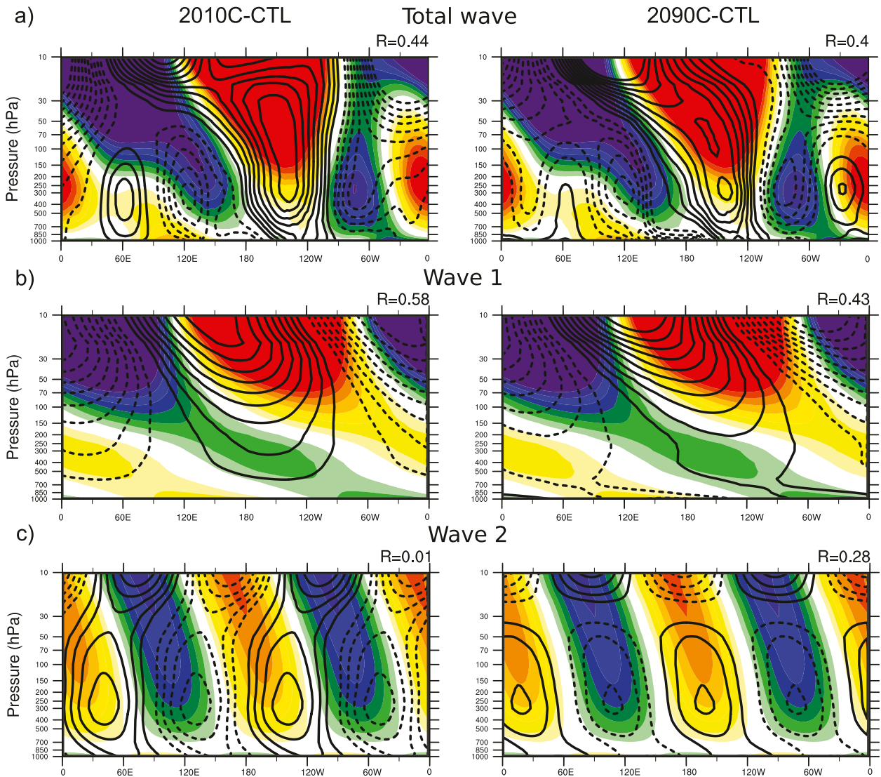
FIG. 11. Forced (contours) and climatological (shading) stationary waves at 60^{\circ}\text{N} in (left) 2010C and (right) 2090C in February. The stationary waves are obtained by removing the zonal mean of the geopotential height. Results are shown in a pressure vs longitude plot for (a) total wave (no Fourier decomposition), (b) zonal wavenumber 1, and (c) zonal wavenumber 2. Spatial correlations between the forced and climatological waves are indicated. Contour interval is 20 m (5 m) for the climatological (forced) waves.
