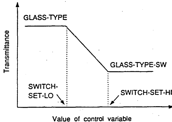
Figure 2.25: Control action for switchable glazing. Glass properties, such as solar transmittance, depend on the value of a user-specified control variable.
