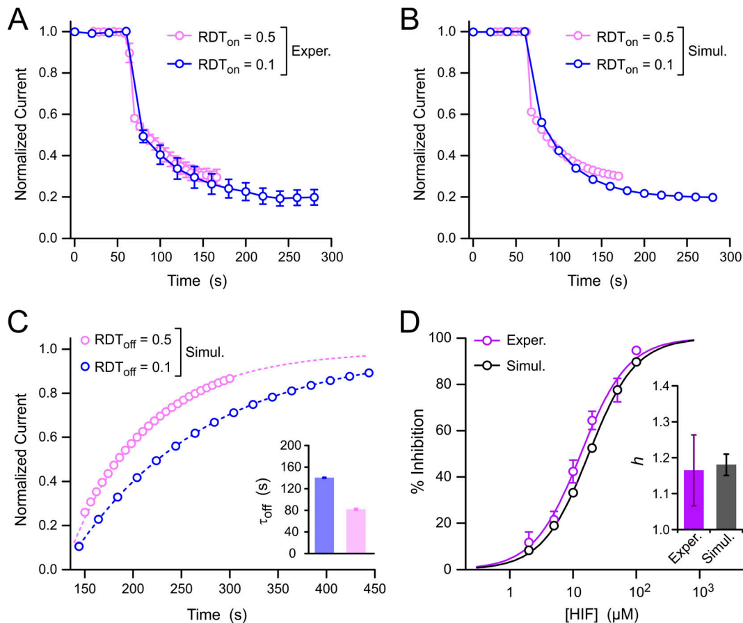
Figure S3. Comparisons between experimental and simulated data using model S. (A and B) Experimental and simulated time courses of HIF-mediated inhibition of Hv1 WT as a function of RDT_{on} . Experimental data are the same as in Fig. 1 B. The recovery from inhibition was omitted for clarity. \tau_{slow} values as a function of RDT_{on} are reported in Fig. 1 C; \tau_{slow, RDT_{on} = 0.1} / \tau_{slow, RDT_{on} = 0.5} = 1.15 \pm 0.20 . Time courses of inhibition reported in B were generated with the four-state model of Fig. S2 A. The simulated data were then fitted with a double-exponential function providing \tau_{slow, RDT_{on} = 0.1} / \tau_{slow, RDT_{on} = 0.5} = 1.03 \pm 0.05 . Hence, \tau_{slow} is only weakly affected by differences in RDT_{on} in both experiments and simulations. (C) Simulated time courses of recovery from inhibition of Hv1 WT as a function of RDT_{off} . Conditions and protocols were as in Fig. S1. Time courses were fitted with a single-exponential function. Time constants from fits are shown in the bar graph ( \pm SE). Simulated currents recover faster when the relative depolarization time increases, as observed experimentally (Fig. S1). (D) Concentration dependence of HIF-mediated Hv1 inhibition simulated with the four-state model of Fig. S2 A shown in black compared with the experimental concentration dependence from Zhao et al. (2021) shown in purple. Each experimental data point represents the mean of three to five independent measurements \pm SD. Simulated and experimental data points were fitted with the Hill equation (Eq. 4). The resulting Hill coefficients ( h ) are compared in the bar graph. Error bars are SE. Simulated half maximal inhibitory concentration ( IC_{50} ) was 17.7 \pm 0.4 \mu M . Experimental IC_{50} was 13.3 \pm 1.0 \mu M (Zhao et al., 2021). The simulated data were generated by applying the same protocols used in the experiments. So, we assume that h > 1 could be due, at least in part, to some imperfect experimental conditions (e.g., not reaching true steady state of inhibition at all concentrations; see Discussion). Exper., experiment; Simul., simulation.
