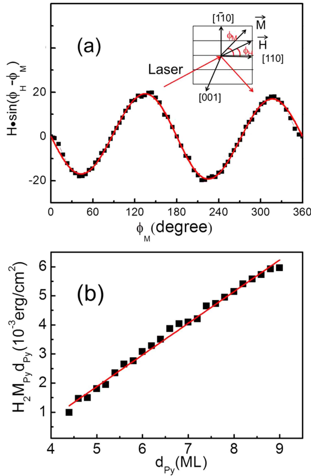
Figure 3. (a) Magnetic torque of H\sin(\phi_H - \phi_M) vs \phi_M from ROTMOKE measurement on vicinal Cu/Py(6ML)/Cu(001). The red line is the fitting result using eqn. (2). (b) The anisotropy field versus Py thickness. A linear fit using eqn. (3) determines the surface and volume parts of the step-induced uniaxial magnetic anisotropy.
