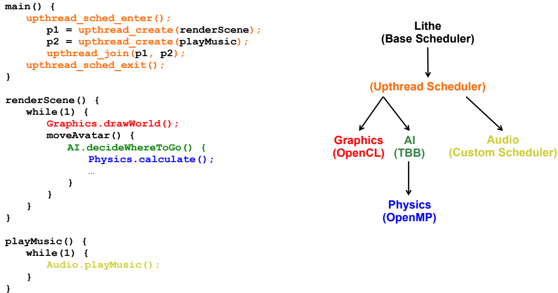
(a) Example program that calls functions inside various lithe-aware runtimes.
