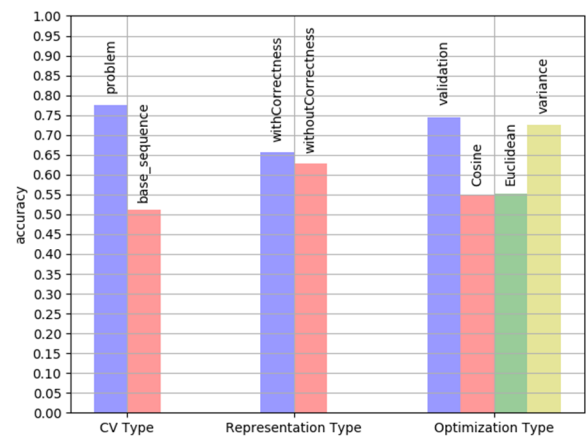
Figure 5: Avg. accuracies from supervised experiments
