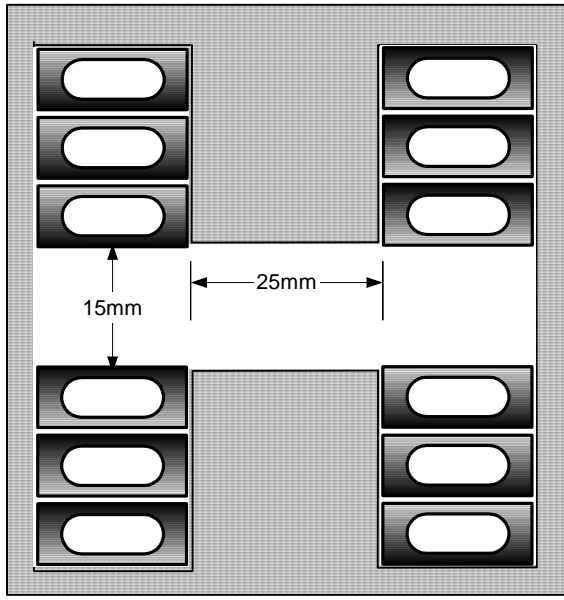
Magnet profile – end view with six water cooled conductors. The full extent of ferrite core is not shown. Fig. 2
