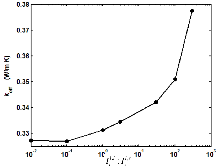
Fig. 12 ETC of three-phase porous media for different liquid-solid phase interaction growth probabilities. The parameters are: \varepsilon=0.5 , c_d=0.01 \varepsilon , P_l=0.3 , k_s=3.0 W/m K, k_l=0.1 W/m K, and k_g=0.025 W/m K.
