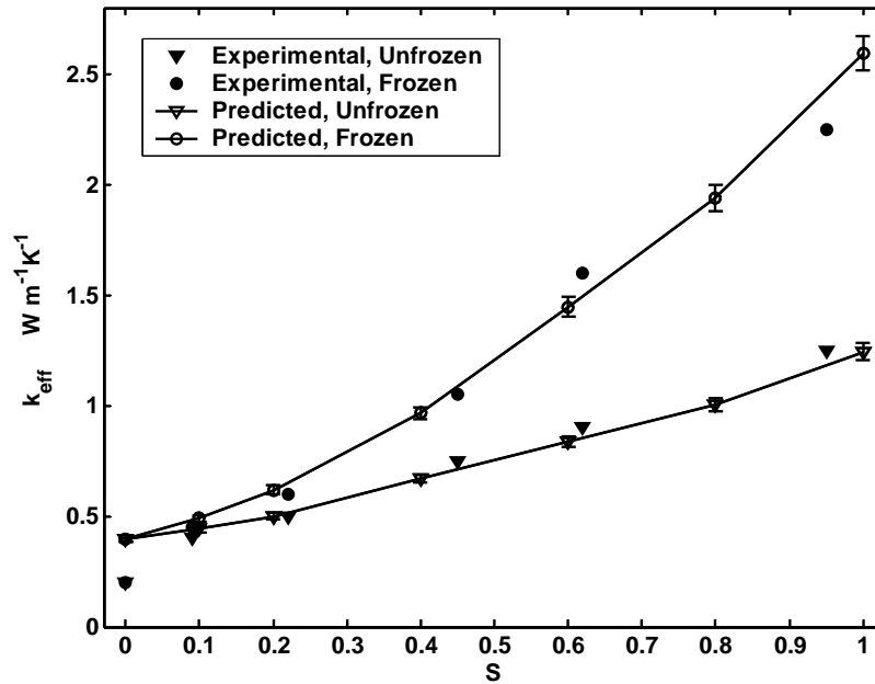
Fig. 4 Comparisons between predicted and experimental effective thermal conductivities of unsaturated porous sands in frozen and unfrozen states. The experimental data is from Ref. [52,53]. The parameters are \epsilon=0.52 , k_s=2.85 W/m·K, k_w=0.5924 W/m·K, k_g=0.0249 W/m·K, and k_{ice}=2.38 W/m·K
