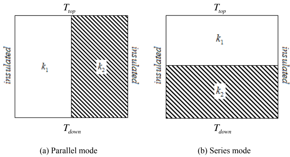
Fig. 2 Two basic structures for validation
