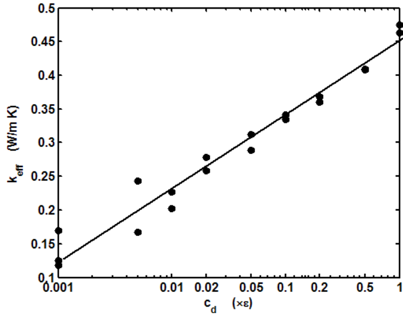
Fig. 7 ETC versus value of c_d at \epsilon=0.5
