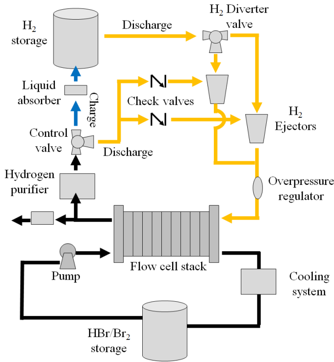
Figure 4. Simplified hydrogen-bromine flow diagram
