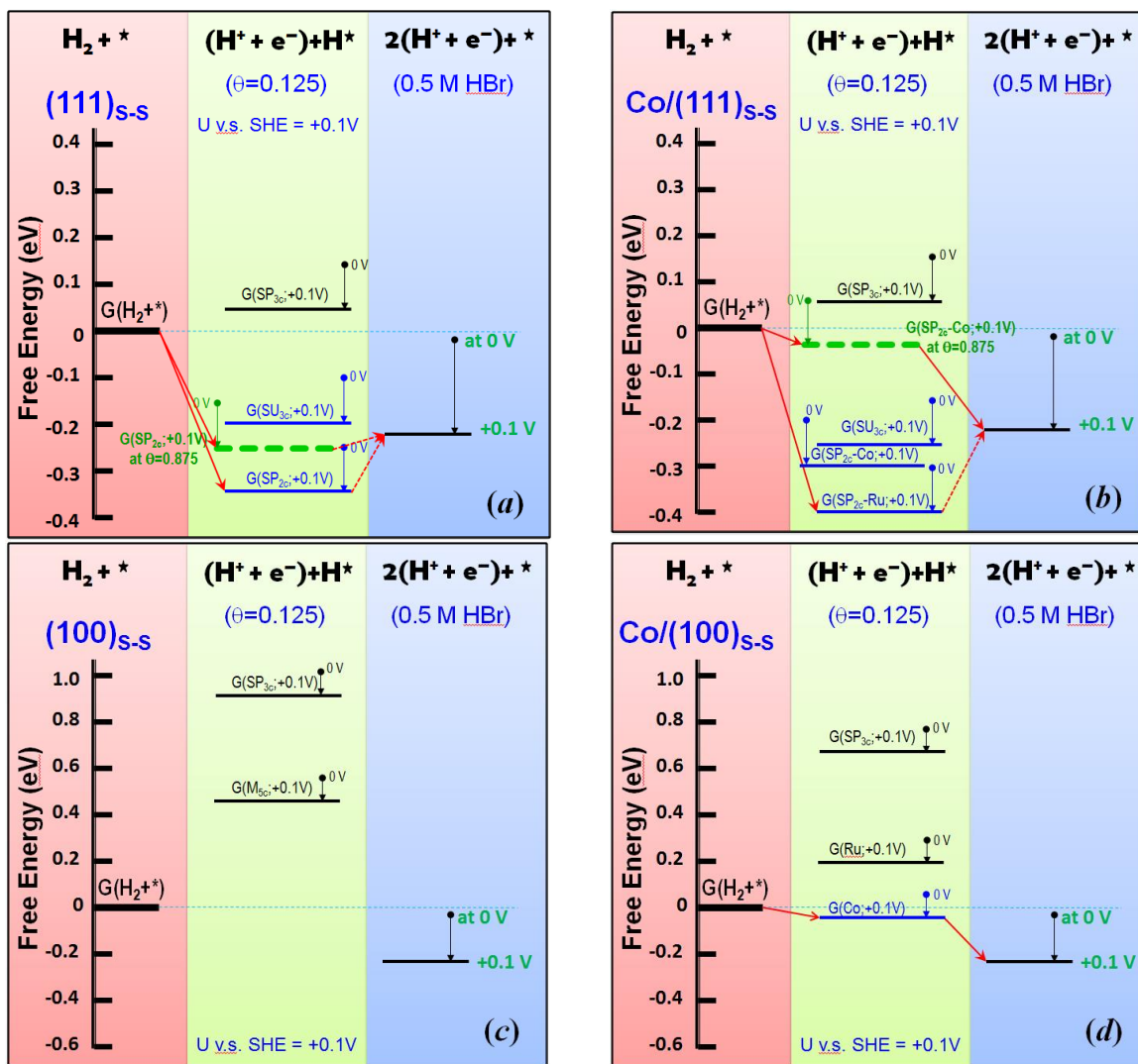
Figure 9. Free energy diagram for HOR ( \text{H}_{2(\text{g})} \rightarrow 2(\text{H}^+ + \text{e}^-) ) in 0.5M HBr, at 298K, 1 bar of hydrogen pressure and at voltage +0.1 Volts. The details are the same in Figure 8.
