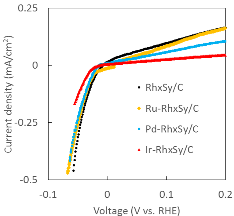
Figure 5. Hydrogen evolution and oxidation activity for 1% Ru, Pd, Ir and pure rhodium sulfide in 1 M \text{H}_2\text{SO}_4 with 1500 rpm rotation. IR compensated and current density based on approximated surface area of the metal sulfide from crystallite size and carbon surface area due to capacitance.
