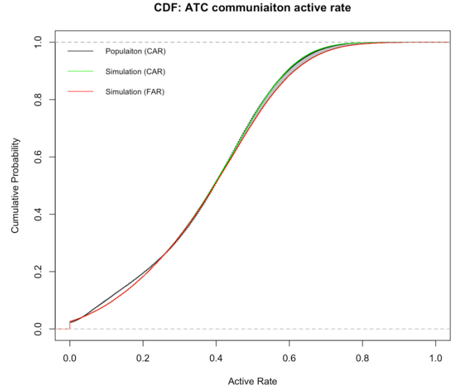
Figure 3. The CDF of Constrained Active Rate and Free Active Rate.
