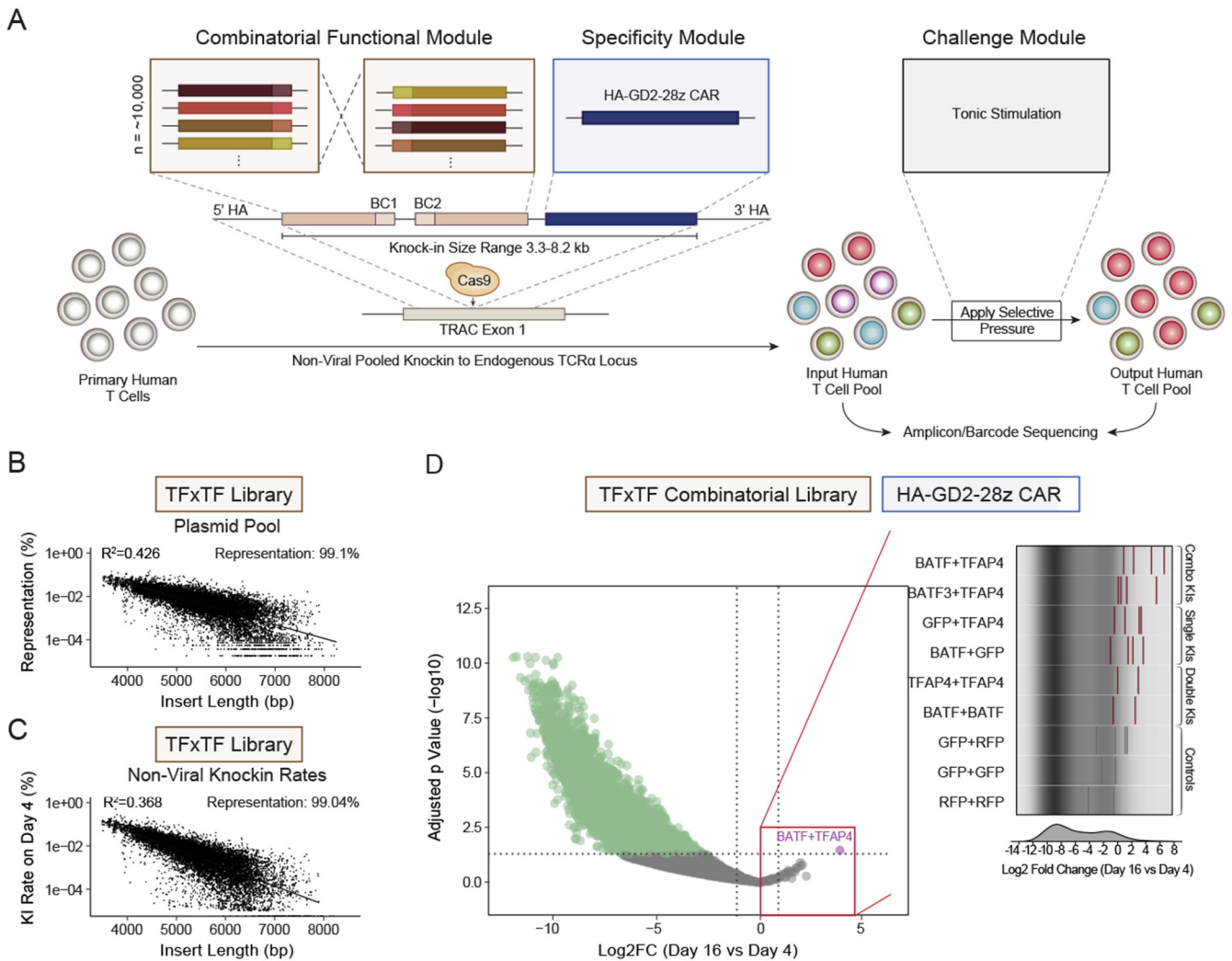
Figure 5. Combinatorial ModPoKI Screens Uncover Efficient TF Combinations
