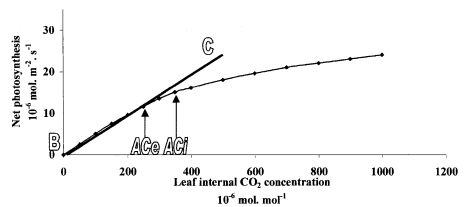
Fig. 1. Schematic representation of an A/C_i curve.
