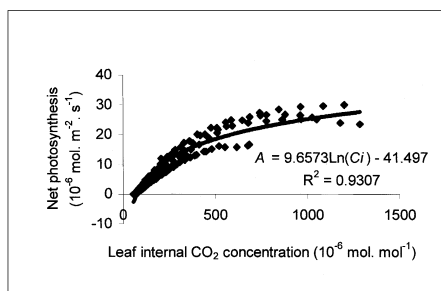
Fig. 2. A/Ci curves of CVC-affected sweet orange plants.
