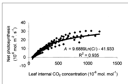
Fig. 3. A/Ci curves of healthy sweet orange plants.
