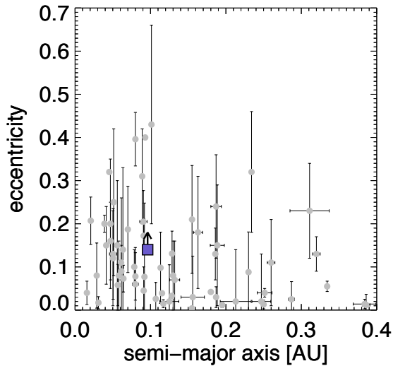
FIG. 9.— Eccentricity vs. semi-major axis for planets in the NASA Exoplanet Archive that have separations less than 0.4 AU, are less massive than Neptune, and have non-zero eccentricities. Our K2-26b 95% confidence lower eccentricity limit is shown as a slate blue square.
