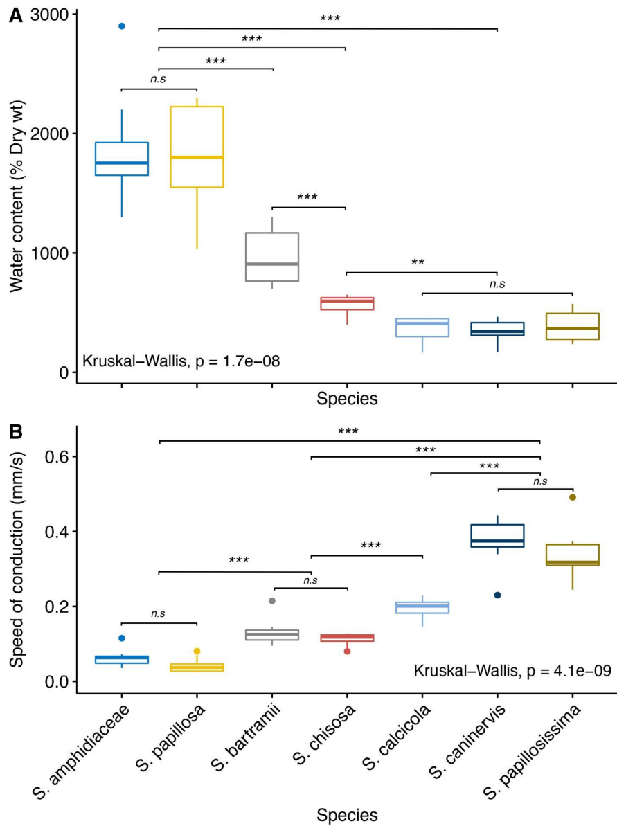
Figure 3.3. Water content (% of dry weight) (A) and speed of external (mm/s) (B) water conduction among different species of Syntrichia .
