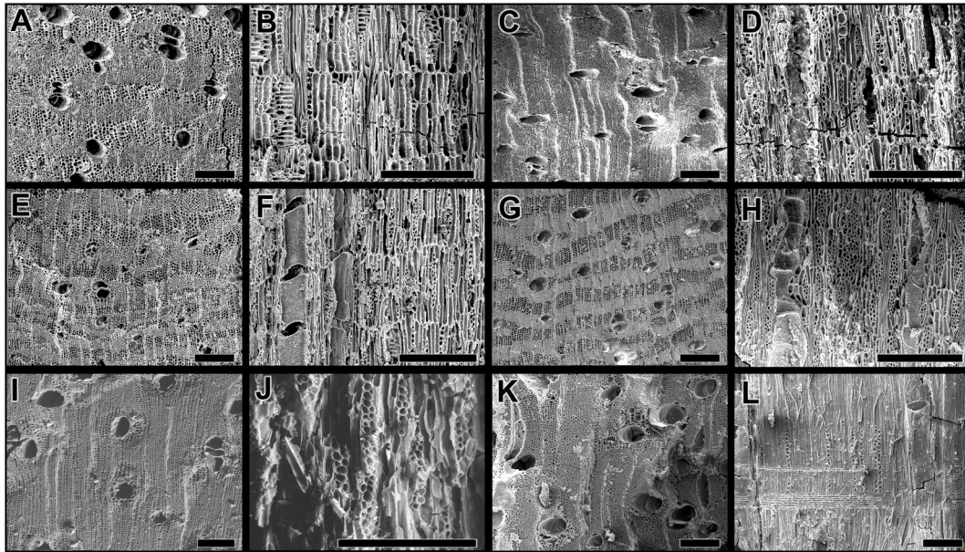
Fig. 2. Scanning electron micrographs of the top six most ubiquitous hardwoods recovered in the form of wood charcoal. A) Haematoxylum campeianum transverse section, B) H. campeianum tangential section, C) Persea americana transverse section, D) P. americana tangential section, E) Crescentia alata transverse section, F) C. alata tangential section, G) Ficus sp. transverse section, H) Ficus sp. tangential section, I) Nectandra sp. transverse section, J) Nectandra sp. tangential section, K) Aspidosperma sp. transverse section, L) Aspidosperma sp. radial section. All scale bars are 200 \mu m.
