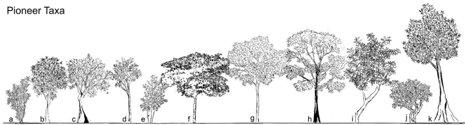
Fig. 6. Arboreal taxa recovered via wood charcoal remains that are indicative of pioneer species that are known to comprise regenerative forests. a) Acnistus aborescens , b) Allophylus sp., c) Casearia sp., d) Exostema caribaeum , e) Matayba sp., f) Muntingia calabura , g) Nectandra cf. globosa , h) Platymiscium sp., i) Psidium guajava j) Tabernaemontana sp., k) Vitex gaumeri .
