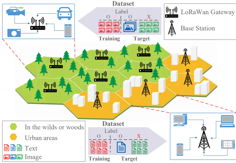
Fig. 1. We consider a scenario where a BS serves a set of devices. The devices each have two datasets, the training dataset and the target dataset. The data points in the training dataset are fully-labeled, whereas those in the target dataset are partially-labeled. Moreover, the number of labeled data points in the target dataset (i.e., the texts and images in blue) is the smallest among the labeled data points in the training dataset (i.e., the texts and images in red) and the unlabeled data points in the target dataset (i.e., the texts and images in green).
