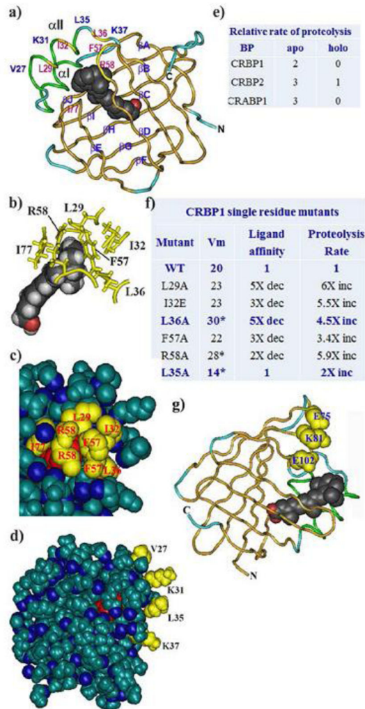
Fig. 7. Structure-activity relationships of retinoid BP. a) Ribbon diagram of CRBP1 illustrating the entrance portal, key residues, orientation of retinol in the binding pocket, and the structure of the \beta -clam (Cowan et al., 1993; Franzoni et al., 2002; Lu et al., 2003; Careri et al., 2006; Mittag et al., 2006; Franzoni et al., 2010; 2016 Silvaroli et al., 2016). Red shows the hydroxyl group of retinol. Structure PDB ID 5HBS, NCBI. b) Partial structure focusing on interactions of entrance portal residues with each other and with the \beta -ionone ring. Red depicts the retinol hydroxyl group. c) Partial space-filling structure illustrating close contacts of residues in the entrance portal. Red illustrates the \beta -ionone ring. d) Total space-filling structure of CRBP1 showing sequestration of retinol from the cellular milieu, and residues that project from the \alpha II helix out from the BP, which serve as putative “handles” that allow enzymes to tease retinol from the BP. Red indicates the \beta -ionone ring. e) Differences in proteolysis rates between apo- and holo-BP. BP were exposed to the endopeptidase Arg-C (clostripain). Degrees of proteolysis were analyzed by SDS-PAGE: scale: 0, no proteolysis; 1, low (<50%); 2, moderate (>50%); 3, complete. These data were obtained after 1 hour incubation, but holo-forms remained protease resistant up to 20 hours (Jamison et al., 1994).
