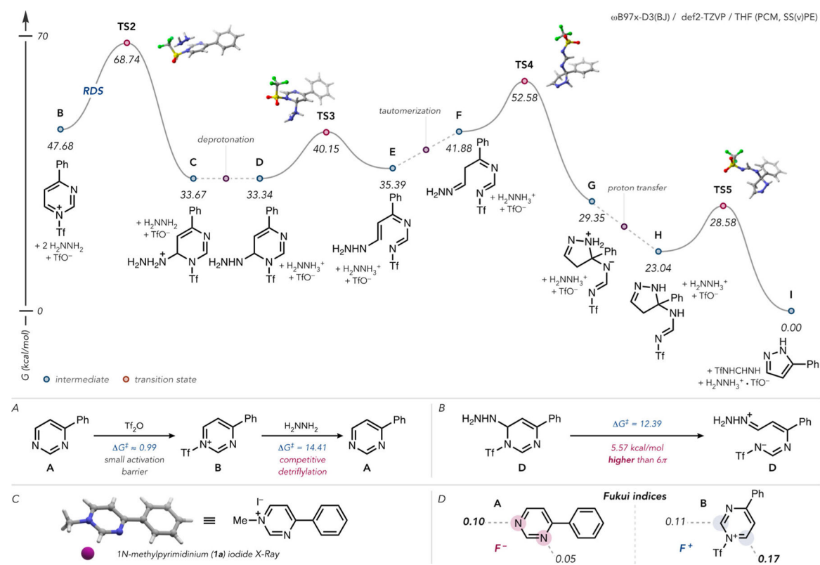
Figure 3. Mechanism of the triflylation-promoted, hydrazine-mediated ring contraction of pyrimidines. (A) Competitive detriflylation of B. (B) Calculations for aminal collapse pathway. (C) X-ray crystal structure of N-methyl-4-phenylpyrimidinium iodide (MeCN molecule omitted for clarity). (D) Fukui nucleophilicity (left) and electrophilicity (right) indices for A and B, respectively.
