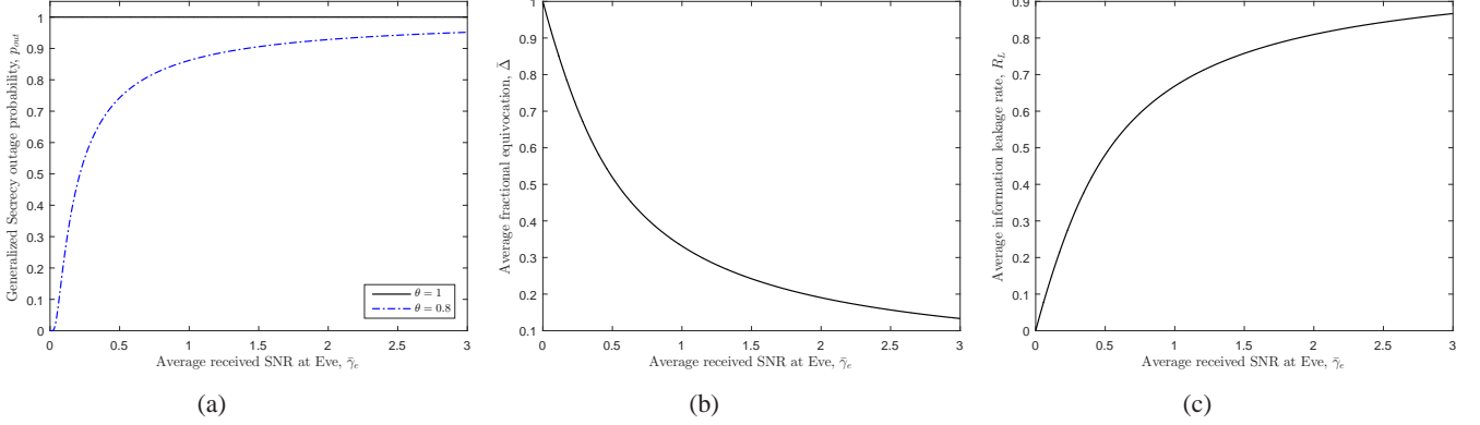
Fig. 5: Secrecy performance versus Eve's channel quality. Results are shown for the transmission with R_b = R_s = 1 . (a) Generalized secrecy outage probability versus average received SNR at Eve. (b) Average fractional equivocation versus average received SNR at Eve. (c) Average information leakage rate versus average received SNR at Eve.
