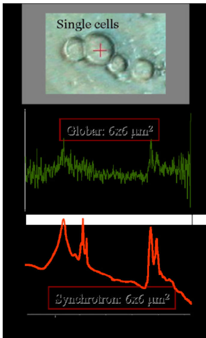
Figure 6. FTIR spectra of a single cell using a 6\ \mu\text{m} \times 6\ \mu\text{m} aperture, comparing results from a synchrotron-based system (red, at Laboratoire pour l'Utilisation du Rayonnement Electromagnétique, Orsay, France) to the spectrum from a lab-based system (green). The collection time for the synchrotron-based system was about 16 seconds (32 scans, bottom), compared to about 500 seconds (1,000 scans, middle) for the lab-based system. These investigators clearly demonstrate that even with significantly longer averaging times, the signal-to-noise of the global measurement is so poor that the data is not usable whereas the synchrotron-based measurements show all the fine spectral structures required for detailed analysis. [Figure courtesy of P. Dumas].
