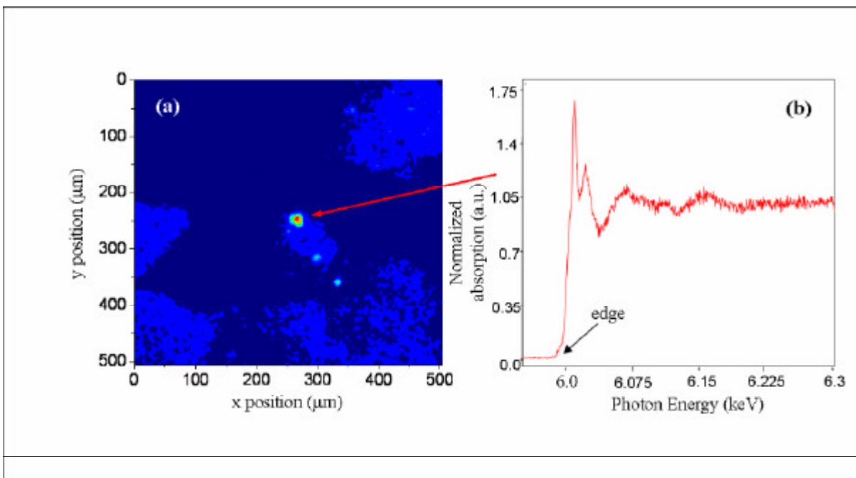
Figure 11. Confirmation of chromium (III) oxidation state by micro-X-ray analysis on the similar area of the identical sample studied by SR FTIR (see Figure 5). (a) Chromium elemental mapping by micro-X-ray fluorescence analysis ( \mu -XRF). The colors go from black (chromium concentration below detection limit) to red (high chromium concentration). (b) Average of 9 micro-X-ray absorption fine structure ( \mu -XAFS) scans taken at the highest concentration spot shows no Cr(VI) pre-edge peak and is consistent with Cr(III) compounds. Each data point represents 20 seconds counting time. The energy increments are 0.5 eV [95].
