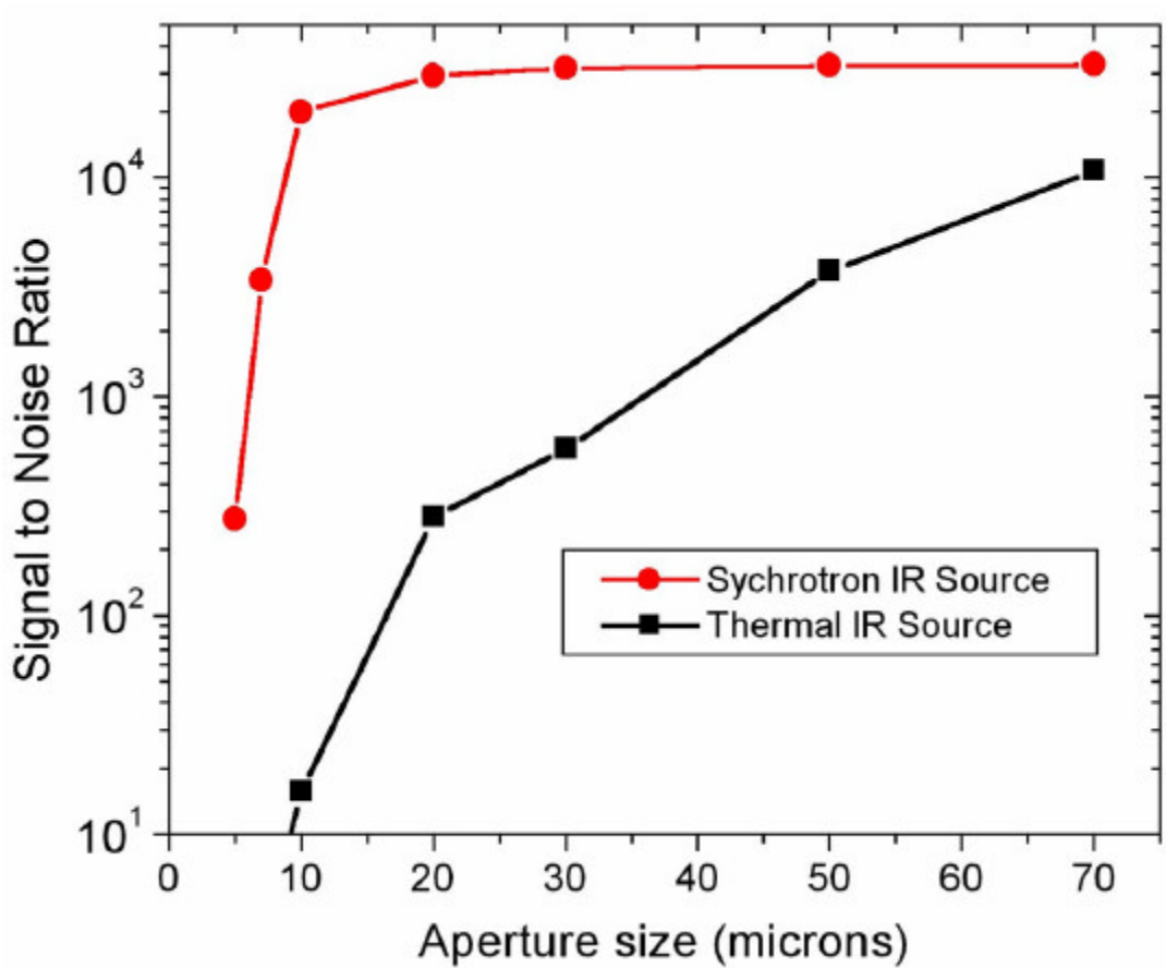
Figure 4. Comparison of measured noise around 100% reflectance for the thermal and synchrotron IR sources with different aperture size expressed in terms of signal to noise ratio on a log scale as a function of aperture size for the synchrotron and thermal IR sources. The synchrotron source extends FTIR spectromicroscopy to below 20 micron spatial resolution with a signal-to-noise advantage over conventional IR sources of at least 100.
