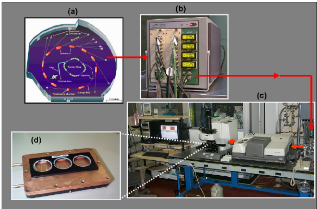
Figure 7. The beam position locking system instrumentation at Beamline 1.4.3 at the ALS. It is specifically made for probing biogeochemical processes in situ and in vivo . The beam from the synchrotron (a) is passed through the beam position locking system (b), then enters the commercially available FTIR spectromicroscopy system (c). During the experiment, samples are kept inside a stage mini-incubator (d). The addition of the beam-locking system is exceedingly helpful when studying biogeochemical materials that often have fine and highly heterogeneous surface features.
