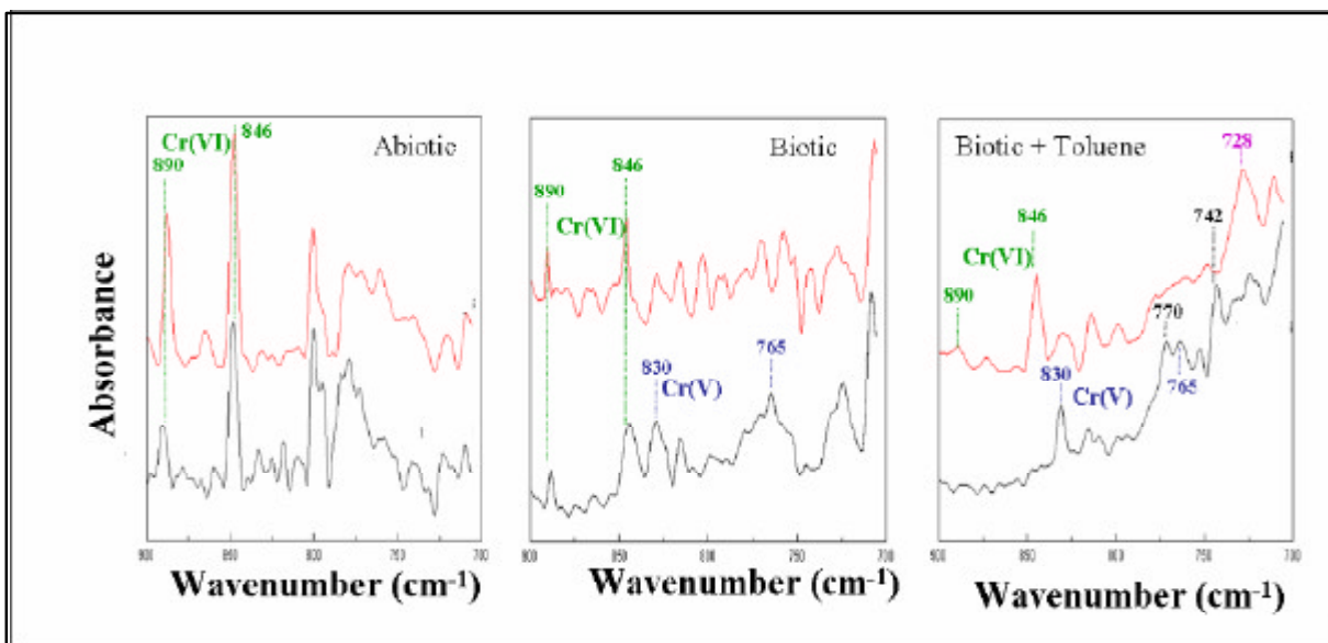
Figure 8. SR-based FTIR spectra of chromate on magnetite surfaces during the 5-day experiment of (left) abiotic reduction, (middle) biotic reduction in the absence of other organic compounds, and (right) biotic reduction in the presence of toluene vapor (as a model volatile organic compound). (—) t < 1 day, shifted vertically for visual clarity. (—) t = 5 days. Although the total chromate concentration for each of the three experiments were the same, microbial-mineral surface roughness and redistribution during evaporation results in heterogeneous spatial distributions of Cr(VI) concentrations. The most relevant vibrational frequencies identified are marked: 890 and 846\text{cm}^{-1} correspond to Cr(VI), 830 and 765\text{cm}^{-1} correspond to Cr(V), 770 and 742 are catechols, and 728 is toluene. We observe that microbial reduction of Cr(VI) is the dominant mechanism in our experimental system. The microbial chromium reduction is further enhanced during the microbial degradation of the organic compound toluene [95].
