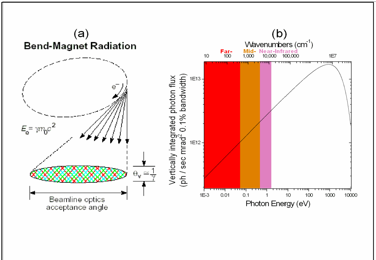
Figure 3. An overview of synchrotron radiation. (3a) Guided by a series of bending magnets and straight sections, relativistic electrons inside a storage ring complete a loop. When the relativistic electrons encounter a magnetic field, they are deflected and they emit electro-magnetic radiation with energy photons up to hard x-rays. (3b) This so-called bending magnet spectrum extends from very low energies (far-infrared) continuously to a critical energy in the soft or hard x-ray, depending on the energy of the synchrotron. The radiation pattern from relativistic electrons is such that its effective source size can be considered as very close to an ideal point source.
