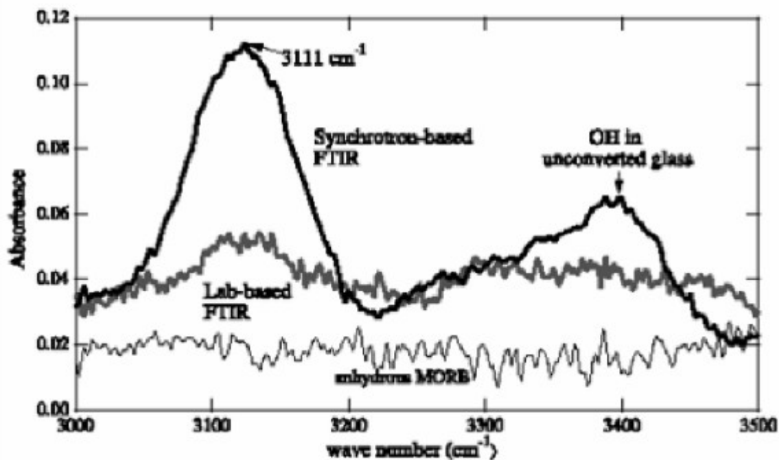
Figure 5. Spectra of a sample synthesized at 32 ( \pm 2 ) GPa and 2850 ( \pm 150 ) K, comparing results from a synchrotron-based system (black, Advanced Light Source beamline 1.4.3; Nicolet Magna 760 with KBr beamsplitter and an MCT detector) to the spectrum from a lab-based system (gray, Bruker IFS-66v using a CaF 2 beamsplitter and an InSb detector). The collection time for the synchrotron-based system was about 2 min (256 scans, top), compared to about 7 hours (60,000 scans, bottom) for the lab-based system. While both show a distinct peak at 3111 \text{cm}^{-1} corresponding to OH vibrations in stishovite, the synchrotron-based spectrum has a better signal-to-noise ratio, as well as better spatial resolution. There is no detectable absorption at 3450 \text{cm}^{-1} , where OH in Mg-perovskite is expected to absorb. A control experiment was performed on a dry, synthetic basalt glass starting material (sample 1114b_6); synthesis conditions were 33 ( \pm 1 ) GPa and 2130 ( \pm 150 ) K. No absorption features were found in the 3000–3500 \text{cm}^{-1} region for this sample (thin line, bottom), again collected by synchrotron FTIR [158].
