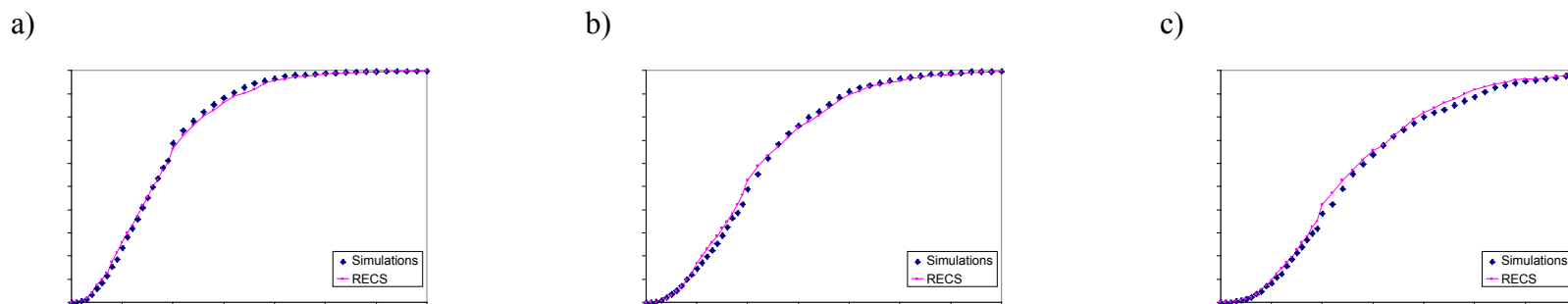
Figure 5.7. Cumulative distributions of electricity use for non-heat pump homes from simulations (blue diamonds) and from RECS (pink lines) in the in the a) smallest 1/3 of homes ( Q_{KS} = 0.721 ) b) middle-sized 1/3 of homes ( Q_{KS} = 0.386 ) and c) largest 1/3 of homes ( Q_{KS} = 0.187 ).
