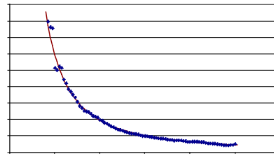
Figure 3.2. a) System curve coefficients of measured home HVAC systems as a function of maximum airflow. B) Smoothed system curve coefficient data as a function of maximum airflow, with the power law fit illustrated.
