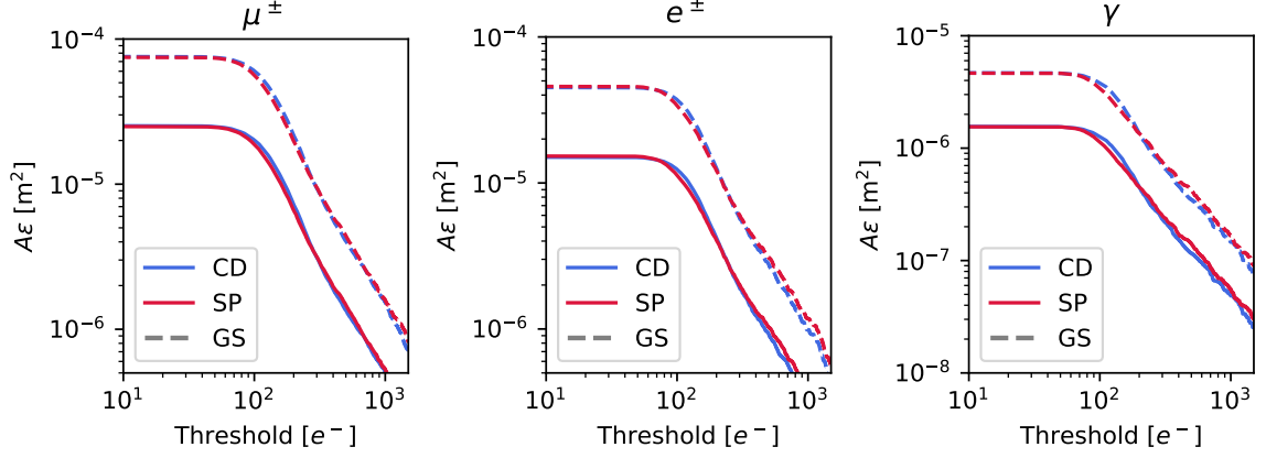
Figure 8.10: Plots of A\epsilon for muons (left), electrons and positrons (middle), and gammas (right, with modified scale) for various sensor trends. The CD sensor is identical to the IMX260 on the Galaxy S7, while the SP sensor has a modified pixel pitch of 0.8\mu\text{m} and a pixel depth of 3.8\mu\text{m} . The GS trend simply scales the areas by a factor of 3.
