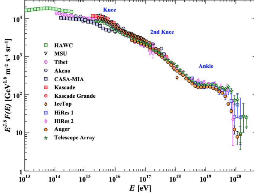
Figure 1.3: The all-particle spectrum from EAS reconstruction, compiled by [53] from [54–64]. The vertical axis has been multiplied by E^{2.6} to better display the features of this steep power-law spectrum.
