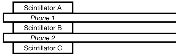
Figure 5.1: A diagram of the hodoscope construction.
