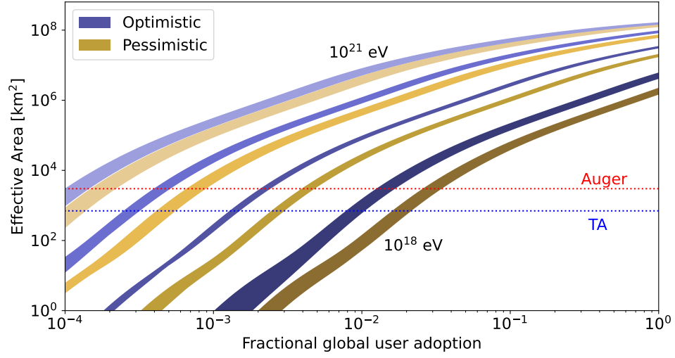
Figure 8.13: The effective area of the CRAYFIS experiment as a function of global user adoption and UHECR energy. The colored bands represent the same parameters as their counterparts in Figure 8.11.
