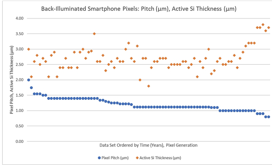
Figure 2.3: Active silicon thickness (orange) and pixel pitch (blue) for devices between 2009-2019. While pixel thickness remained roughly constant for devices up to the 1.12\text{ }\mu\text{m} generation, more recent sensors boasting sub-micron pixels have extended the pixel thickness to increase FWC. From Ref. [118].
