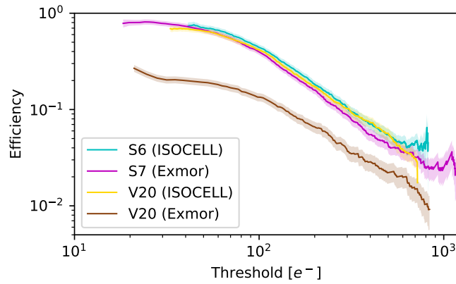
Figure 5.26: Agreement between efficiencies in Figures 5.24 and 5.25. The top S6 and bottom S7 are plotted with the two V20s.
