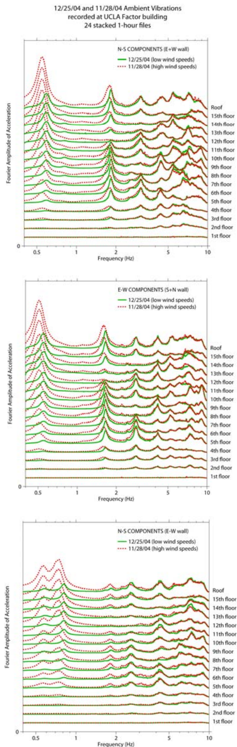
Figure 2: Ambient vibration Fourier amplitude spectra recorded on 12/25/04 (a low wind speed day: solid curves) and 11/28/04 (a high wind speed day: dashed curves).
