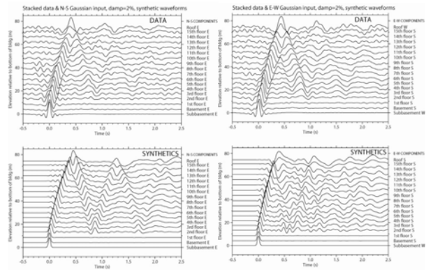
Figure 4: Stacked impulse response functions for the north-south (left, top) and east-west (right, top) components, and associated synthetic waveform results (bottom) using the ETABS modeling for a Gaussian input with 2% damping.
