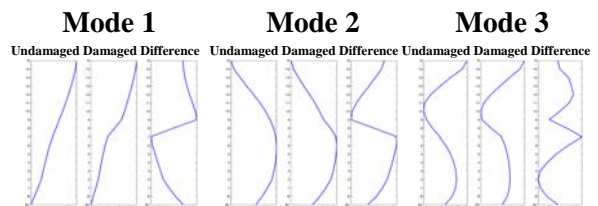
Figure 6: Synthetic mode shapes from a hypothetical damage pattern that simulates broken welds on the 8 th floor. The “Damaged” plots are for the model that simulates the broken welds. The “Difference” plots have been scaled by a normalization factor.
