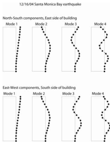
Figure 5: Mode shapes determined from observed displacements (filled circles) at the Factor building during the 12/16/04 Santa Monica Bay earthquake (distance=35 km, M_L=3.6 ).
