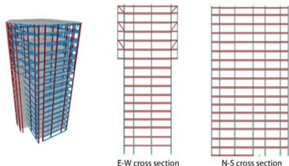
Figure 3: The ETABS model of the Factor building showing the primary major structural elements, and cross sections of major structural elements.
