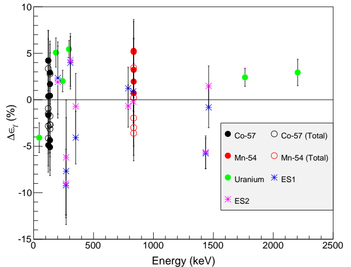
FIG. 5. Percent differences between the measured and simulated \gamma -ray efficiencies as a function of \gamma -ray energy. The simulated efficiencies were obtained using the adjusted values in Table IV. Points corresponding to total efficiencies are indicated with “(Total)” in the legend. All other points correspond to peak efficiencies.
