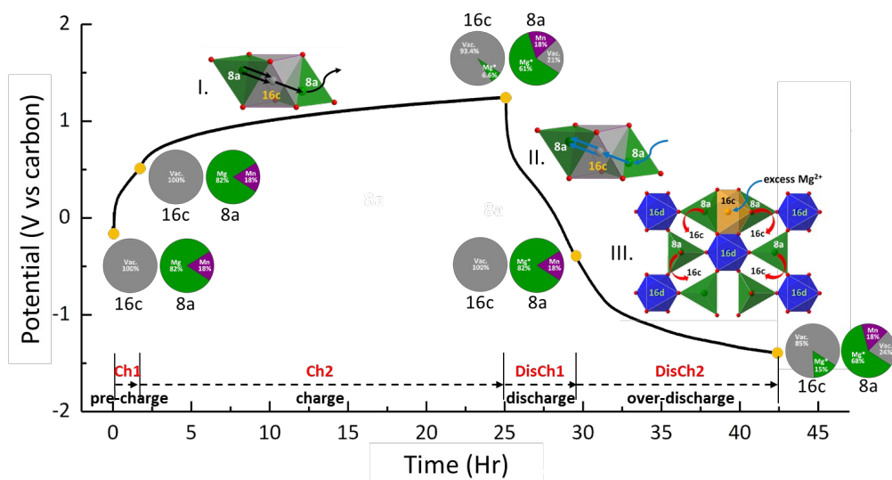
Fig. 6 Schematic illustration of three cation migration processes of the inverted \text{MgCrMnO}_4 during the first charge/discharge. Pie charts represent the fractions of cations on the 8a and 16c sites at the selected state of charge.
