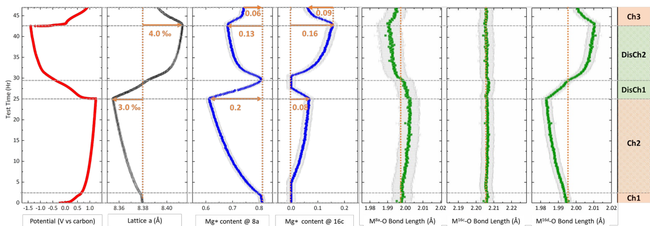
Fig. 4 Structural parameters (lattice parameter, \text{Mg}^* contents and M-O bond lengths) from Rietveld refinements against operando XRD data with the electrochemical curve (V vs. activated carbon) on the left. The \text{Mg}^* contents at 8a, 16c sites are x and y in [\text{Mg}_x\text{Mn}_{0.18}]^{\text{8a}}[\text{Mg}_y]^{16\text{c}}[\text{CrMn}_{0.82}\text{Mg}_{0.18}]^{16\text{d}}\text{O}_4 , respectively. Ch1, Ch2, DisCh1, DisCh2 and Ch3 correspond to five stages of structural evolutions during the operando measurement.
