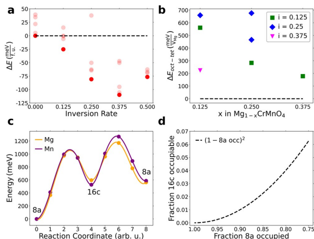
Fig 5. (a) Energies relative to the pristine (zero inversion) \text{MgCrMnO}_4 . At each inversion rate, several cation orderings were sampled, with the lowest energy shown by the fully shaded circles. Energies are normalized per \text{MgCrMnO}_4 formula unit (f.u.); (b) Comparing the energy of Mg extraction from either the 8a site (tet) or 16d site (oct) at varying levels of inversion, i . Energies are normalized per Mg extracted ( V_{\text{Mg}} ) from the \text{Mg}_x\text{CrMnO}_4 supercell with 32 oxygen anions. Positive values indicate a preference for removal from the tetrahedral site; (c) NEB pathway for vacancy-mediated diffusion along the 8a-16c-8a trajectory for Mg and Mn cations; (d) The fraction of 16c sites that are occupiable, as defined by being surrounded by two 8a vacancies, as a function of 8a occupation.
