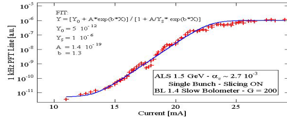
Figure 6: CSR intensity as a function of the current per bunch with the ‘double’ momentum compaction lattice.
