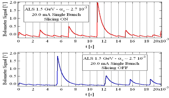
Figure 4: Bolometer signal with the double momentum compaction lattice and above the MBI current threshold. Top: slicing on; bottom: slicing off.
