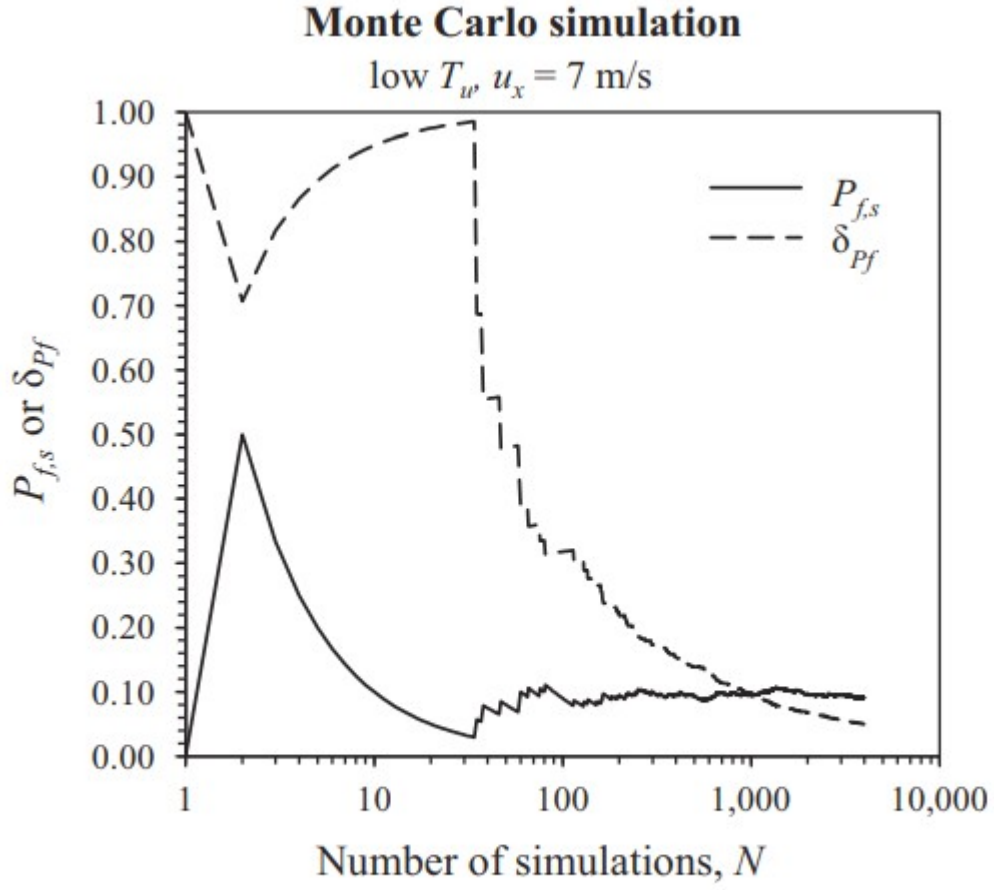
Fig. 10. Evolution of P_{f,s} and \delta_{Pf} for u_x=7 m/s simulation.
