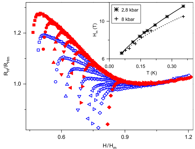
Fig. 2. Scaling of the Hall coefficient R_H/R_{H_m} vs. H/H_m at the pressure of 2.8 kbar (full symbols) and 8 kbar (open symbols). [ H_m, R_{H_m} ] corresponds to the minimum of R_H(H) . Inset: temperature dependence of the scaling field H_m . Solid and dotted lines are power law fits for the data at 2.8 and 8 kbar.
