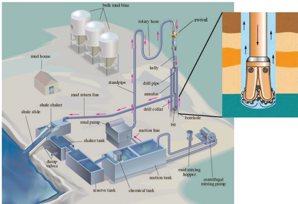
Figure 2-4. Drilling mud circulation system. Arrows indicate mud flow direction (modified from Macini (2005a) and Oil Spill Solutions (2014))
