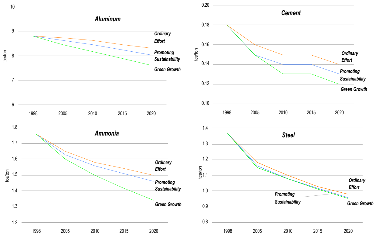
Figure 12. Primary energy intensities of major industrial products will decline, approaching levels currently prevailing in industrialized countries. Most opportunities for greater efficiency are presumed to be taken in the steel industry, even under Ordinary Effort.
