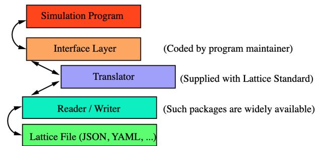
Figure 3: Schematic showing how a simulation program can interact with a PALS compliant lattice file.
