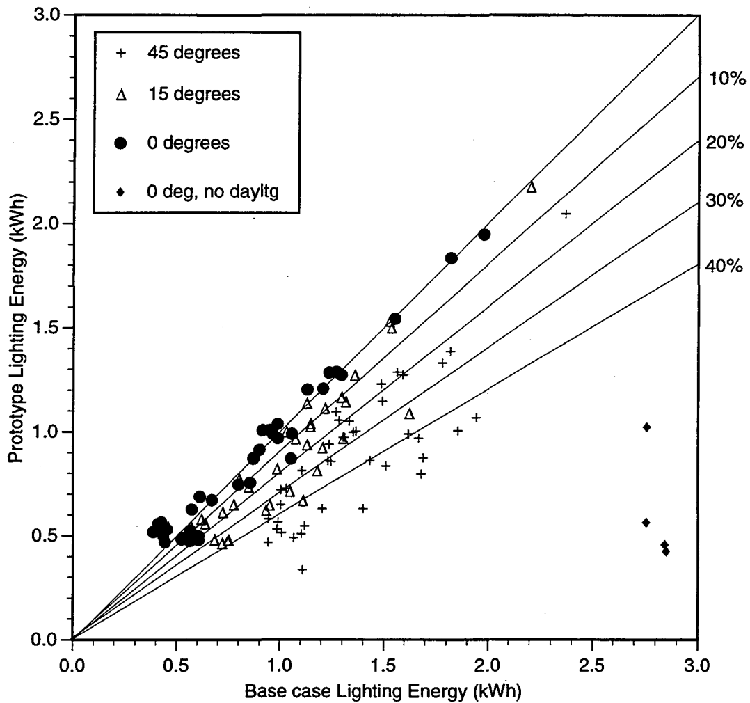
Fig. 6. Daily lighting load (kWh) of the base case and prototype venetian blind/ lighting systems, where the base case was defined by three static blind angles, 0° (horizontal), 15°, and 45°. Diagonal lines on the graph show percentage differences between the base case and prototype. Both cases were defined by the prototype continuous dimming lighting control system or, within a limited set of tests, the lighting control systems with no dimming controls ("no daylight"). Lighting power density is 14.53 W/m 2 (1.35 W/ft 2 ), glazing area is 7.5 m 2 (80.8 ft 2 ), and floor area is 16.96 m 2 (182.55 ft 2 ). Data collected from June 1996 to August 1997. Measurement error between test rooms is 12±46 Wh (2.6±5.4%).
