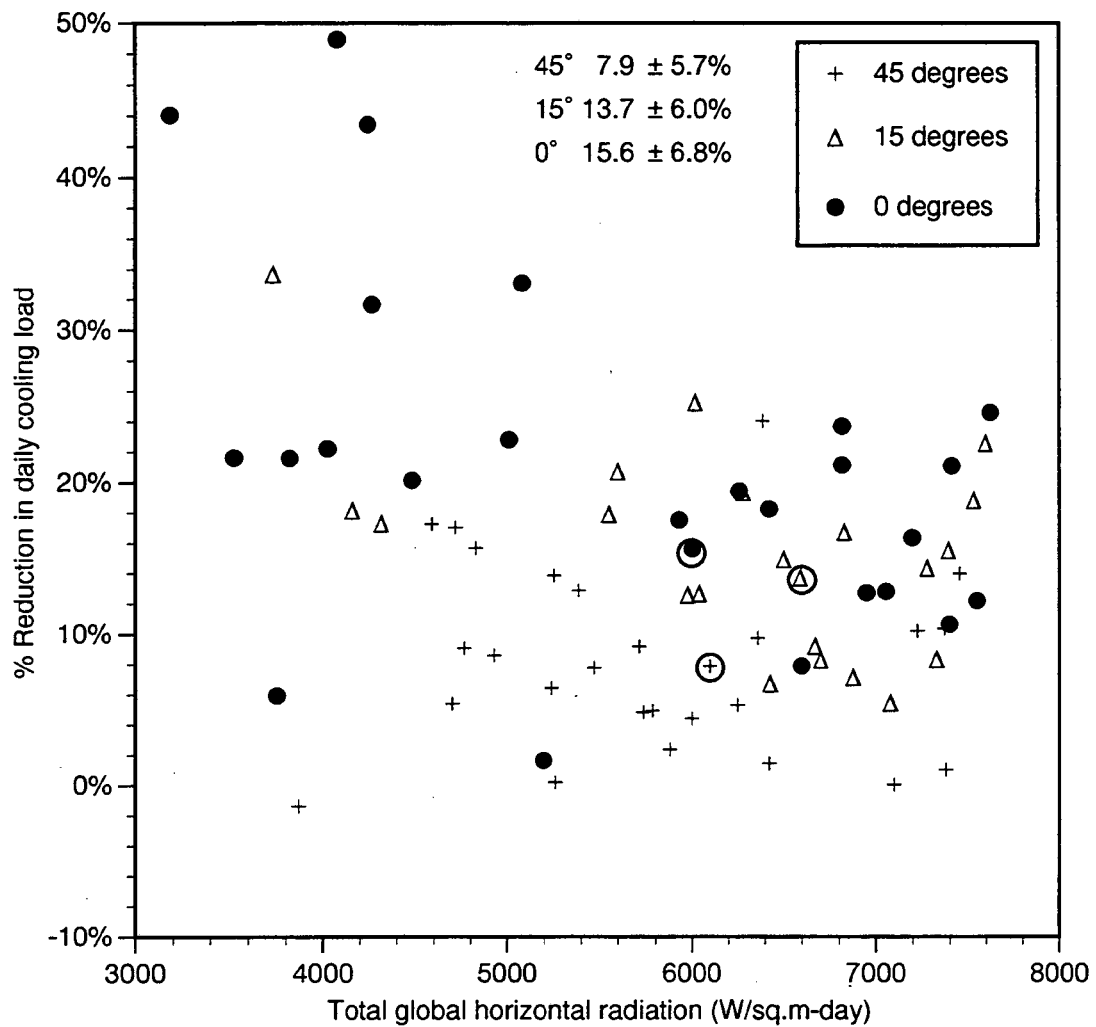
Fig. 13. Percent reduction in daily cooling load compared to the base case static venetian blind with the same dimmable prototype lighting control system as a function of total daily global horizontal radiation (W/m 2 -day). All daily cooling loads greater than 5 kWh. Average values shown circled on graph.
