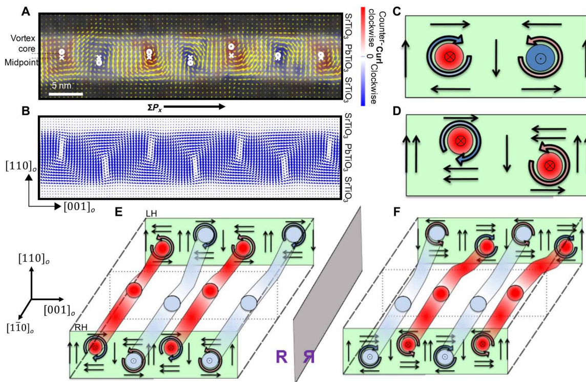
Fig. 1. Different mechanisms for achieving chirality. (A) HAADF-STEM displacement map of polar vortex array. Colors indicate the curl of the local polarization. Circles represent the core of the vortices, and crosses represent the center points of the \text{PbTiO}_3 layer. (B) Phase-field modeling of vortex array demonstrating pronounced buckling of vortices. (C) CW (blue curled arrow) and CCW (orange curled arrow) vortices coupled with antiparallel axial components of the polarization. Filled red and blue circles represent the direction of the axial polarization (along the [1\bar{1}0]_o direction), and light colors represent lower values. Straight arrows represent the direction of the local polarization along the [001]_o (horizontal) or [110]_o (vertical) directions. Within the right-hand rule discussed in (20), both vortices in the sketch are right handed. (D) Asymmetry between up- and down-polarized domains (along [110]_o ), superimposed on an offset that generates a mismatch between left and right polarization along the [001]_o direction. In the sketch, at the center of the ferroelectric layer, the two vortices point predominantly to the left. The handedness of the two vortices is opposite, but one of them is slightly larger than the other, giving the whole system a net chirality. (E) Schematic representation of the right-handed and left-handed domains experimentally observed, separated by a domain wall (dashed square at the center). The two sources of chirality (antiparallel axial components at the center of consecutive vortices plus an offset of its center) coexist within a domain. At the domain wall, the sense of rotation of a vortex is reversed, keeping constant the sense of the axial polarization. (F) Vortices of (E) after performing a mirror symmetry operation, represented by "R." Schematics with the three orthogonal reflections of the polar texture supercell to determine their chiral nature are presented in fig. S1.
