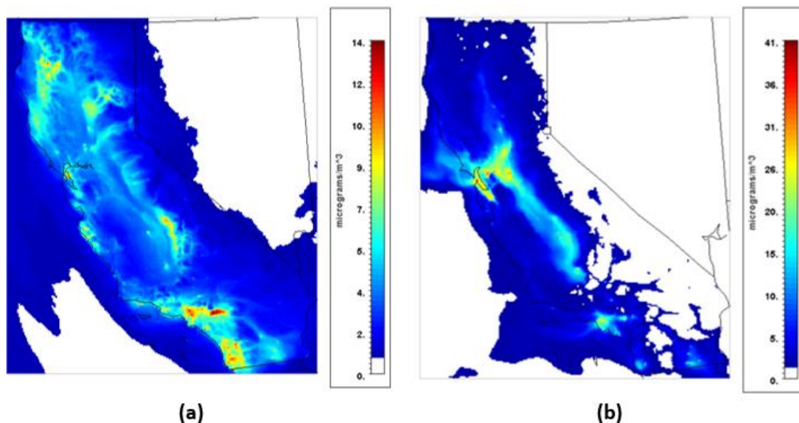
Figure 29. Ambient 24-hr \text{PM}_{2.5} in the SIP Case for (a) Summer and (b) Winter in the SIP Case
