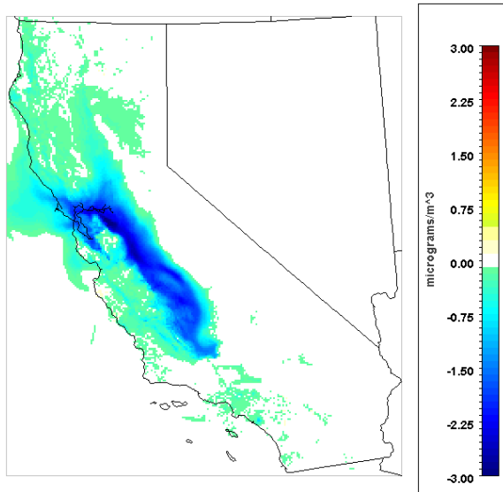
Figure 23. Predicted difference in winter episode 24-hr average PM_{2.5} for Case 2B relative to the Base Case
