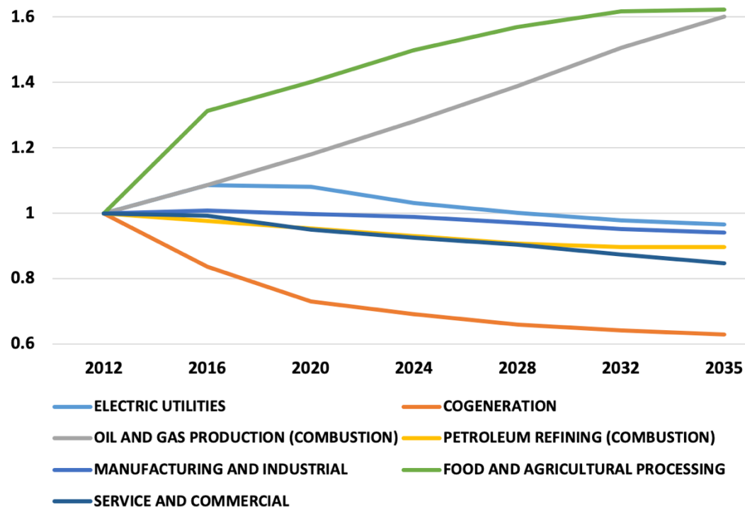
Figure 11. Normalized \text{NO}_x emissions from stationary fuel combustion in California. From Reference [21].
