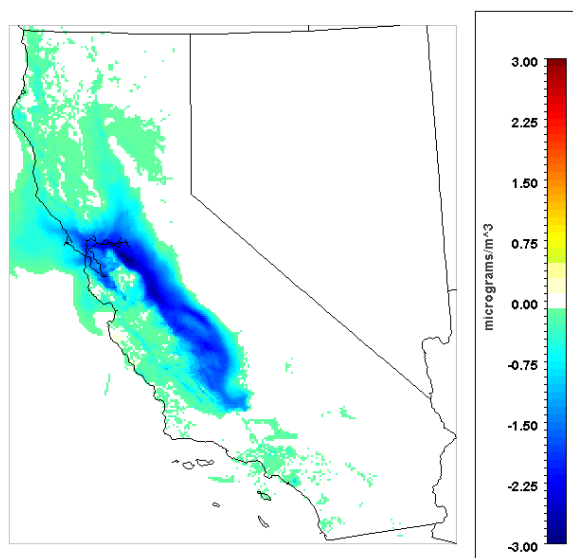
Figure 23 displays the predicted difference in 24-hr PM_{2.5} between the Base and 2B Case for the winter episode. Improvements in ground-level PM_{2.5} are significant with reductions reaching -6.26 \text{ ug/m}^3 and -3.36 \text{ ug/m}^3 in maximum 1-hr and 24-hr average, respectively.
