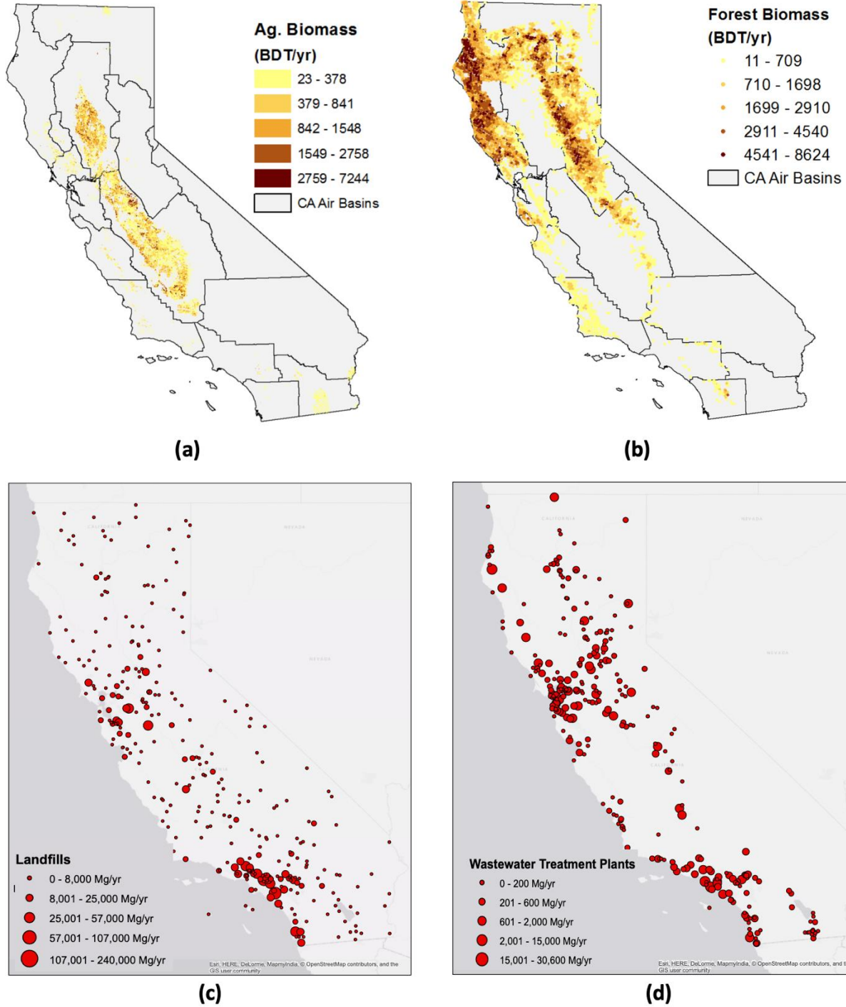
Figure 10. (a) Agriculture biomass in CA in bone dry ton (BDT) per year. (b) Estimate of forest biomass residue in CA in BDT per year. (c) Currently available biomethane in CA from landfills in megagrams (Mg) of Methane per year. (d) Currently available biomethane in CA from wastewater treatment plants in Mg of Methane per year.
