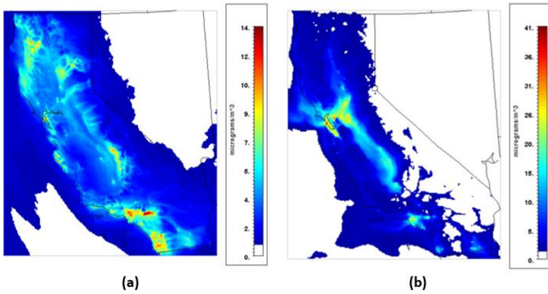
Figure 29 shows the predicted 24-hr average PM_{2.5} for the summer (
