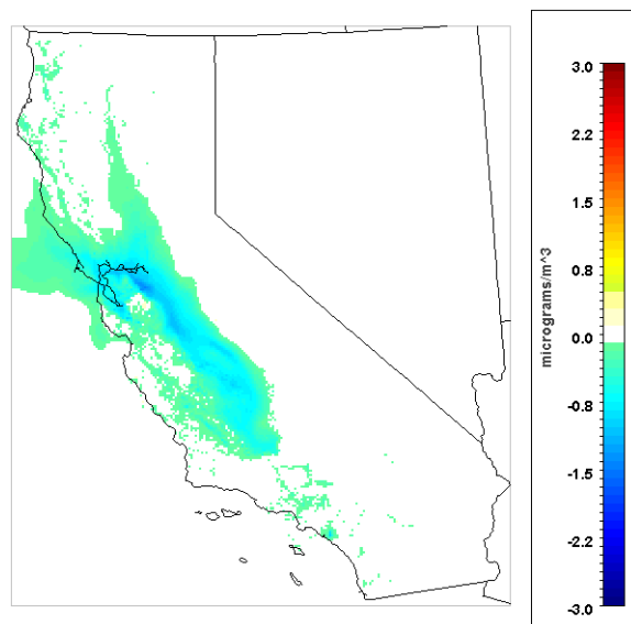
Figure 39 displays the predicted difference in 24-hr PM 2.5 between the SIP and 4A Case for the winter episode. Improvements in ground-level PM 2.5 reaching -5.75 ug/m³ and -1.41 ug/m³ in maximum 1-hr and 24-hr average, respectively.
