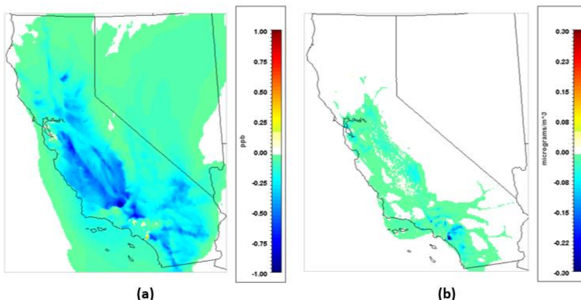
Figure 38 displays the predicted difference in maximum 8-hour ozone and 24-hour PM_{2.5} between the SIP and 4A Cases for the summer episode. Reductions in ozone reach -2.15 ppb and -1.16 ppb in maximum 1-hr and 8-hr average, respectively. Reductions in PM_{2.5} reach -1.13 \mu g/m^3 and -0.50 \mu g/m^3 in maximum 1-hr and 24-hr average, respectively.
