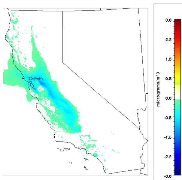
Figure 37 displays the predicted difference in 24-hr PM_{2.5} between the SIP and 3A Case for the winter episode. Improvements in ground-level PM_{2.5} reaching -5.75 \mu\text{g}/\text{m}^3 and -1.42 \mu\text{g}/\text{m}^3 in maximum 1-hr and 24-hr average, respectively.
