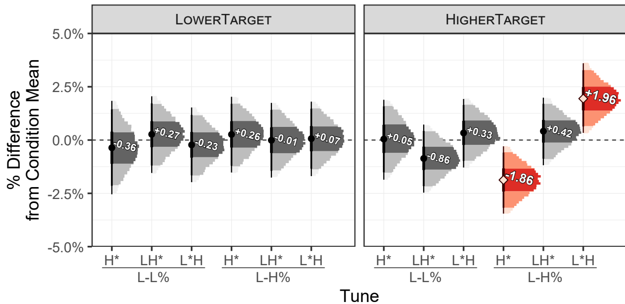
Figure 4: Posterior distribution of RT percent changes with 50%, 89%, and 95% mean highest density intervals. Tunes that are not credibly different from the condition means are shown in gray (means=black circles) while tunes that are credibly different are shown in red (light diamonds).
