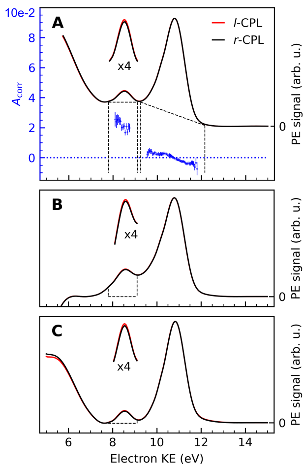
Fig. 2 Background-corrected photoemission spectra of (1S,4R)-(+)-fenchone measured at 301 eV with l - and r -CPL. Panels (A) to (C) show the results of various models by which to subtract the background contribution from a pair of spectra; spectra in Fig. 1 were instead displayed as measured for l -CPL. Background contributions were calculated by (A) fitting an exponential function to the high kinetic end of the spectrum, and subtracting an additional linear background ('roi'-approach); or (B) by fitting a linear combination of an exponential and a linear function to the high- and low-KE ends of the spectra ('exp'-approach). For (C), an exponential function has been fitted and subtracted from the raw data. Then, the 'total background' function 62 is applied to the remaining spectrum ('sum'-approach). Blue points in panel (A) indicate the experimental asymmetries, A_{\text{corr}}(130^\circ) (plotted versus the left y-axis) for the peaks originating from C=O and C-H K-edge photoionization, obtained as the difference divided by two times the mean of r - and l -CPL (eqn (2)), together with associated error bars. The areas marked with dashed lines in panels (B) and (C) indicate the width of the C=O peak, which is used for the asymmetry calculations. Expanded ( \times 4 ) views of these peaks are drawn above the full spectra to get a clearer view on the magnitudes of the l-r asymmetry.
