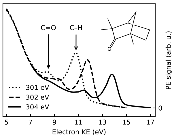
Fig. 1 Electron spectra recorded after photoionization of (1S,4R)-(+)-fenchone with l -CPL at photon energies of 301 eV, 302 eV, and 304 eV; dotted, dashed, and solid lines, respectively. Spectra averaged over a number of sweeps performed at the respective photon energy are shown; no further normalization has been performed. See text for details.
