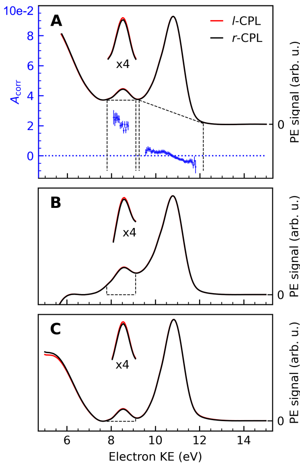
Fig. 2 Background-corrected photoemission spectra of (1S,4R)-(+)-fenchone measured at 301 eV with l - and r -CPL. Panels (A) to (C) show the results of various models by which to subtract the background contribution from a pair of spectra; spectra in Fig. 1 were instead displayed as measured for l -CPL. Background contributions were calculated by (A) fitting an exponential function to the high kinetic end of the spectrum, and subtracting an additional linear background ('roi'-approach); or (B) by fitting a linear combination of an exponential and a linear function to the high- and low-KE ends of the spectra ('exp'-approach). For (C), an exponential function has been fitted and subtracted from the raw data. Then, the 'total background' function 62 is applied to the remaining spectrum ('sum'-approach). Blue points in panel (A) indicate the experimental asymmetries, A_{\text{corr}}(130^\circ) (plotted versus the left y-axis) for the peaks originating from C=O and C-H K-edge photoionization, obtained as the difference divided by two times the mean of r - and l -CPL (eqn (2)), together with associated error bars. The areas marked with dashed lines in panels (B) and (C) indicate the width of the C=O peak, which is used for the asymmetry calculations. Expanded ( \times 4 ) views of these peaks are drawn above the full spectra to get a clearer view on the magnitudes of the l-r asymmetry.
