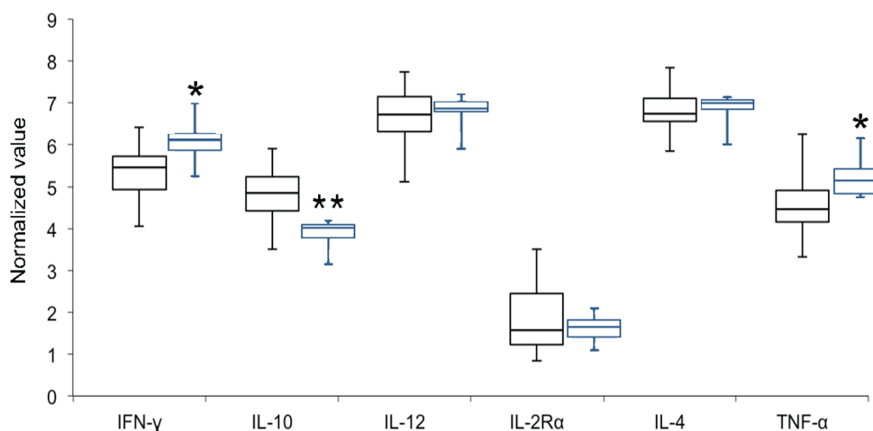
Fig. 1. Box plot of normalized value of 6 immunologically relevant genes for healthy samples ( n=24 , black) and noise-exposed samples ( n=6 , blue). Significant differences between the two sample groups are indicated by stars (* P<0.05 ; ** P<0.01 ). Standard deviation/coefficient of variation of tested genes for healthy samples: IFN \gamma 0.68/0.13, IL-10 0.64/0.13, IL-12 0.76/0.12, IL-2R \alpha 0.76/0.41, IL-4 0.50/0.07 and TNF \alpha 0.74/0.16.
