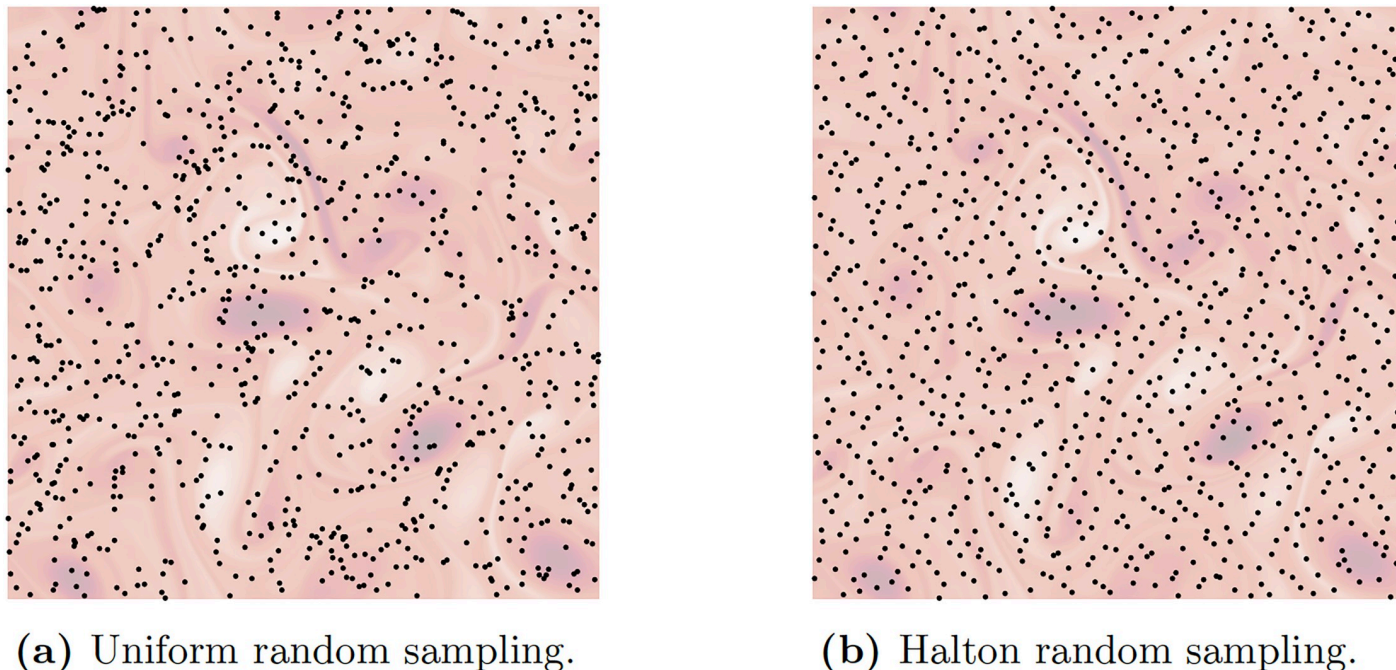
Fig 2. Examples of two different random sampling approaches based on uniform sampling and Halton random sampling. Halton sampling provides a better coverage of the domain than uniform sampling does.
