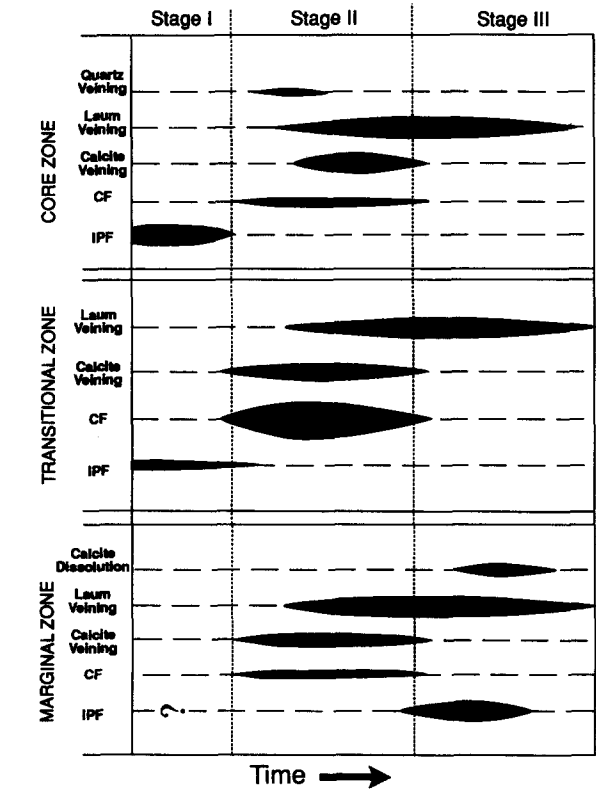
Fig. 10. Relative timing of the different microstructures in the northern marginal, transition and core zone regions of the Duck Creek mélangé. Similar lateral changes are observed across the exposed portions of the southern margin of the diapir. CF = cataclastic floor.
