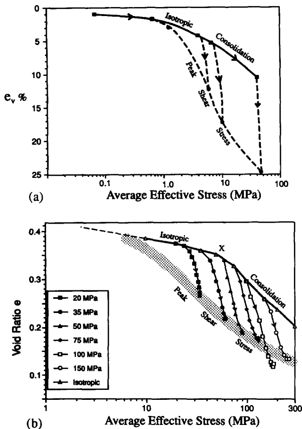
Fig. 13. (a) Influences of shear stress on volume changes associated with crushing of sand grains adapted from Bishop (1966). Average effective stress ((\sigma_1' + \sigma_2' + \sigma_3')/3) plotted against volume change. The sheared Ham River sand samples undergo appreciable grain crushing and further volume reduction over that observed in isotropically consolidated samples except at low confining stresses ( <1 MPa). (b) Data from Zoback & Byerlee (1976) from deformed Ottawa sand. The data is reworked (after the style of Bishop 1966) to show void ratio change against average effective stress for isotropically consolidated and sheared samples. X marks the onset of cataclasis in the isotropically consolidated sample. The effective confining stress for each of the sheared samples is shown. An extrapolation (stippled line) of the void ratios at the peak shear stress suggests that grain crushing becomes significant during shearing of Ottawa sand at average effective confining stresses above 3–7 MPa (depending on the form of extrapolation used). The main thrust of our argument is that the onset of grain breakage occurs at relatively low effective confining stresses in sheared sands.
