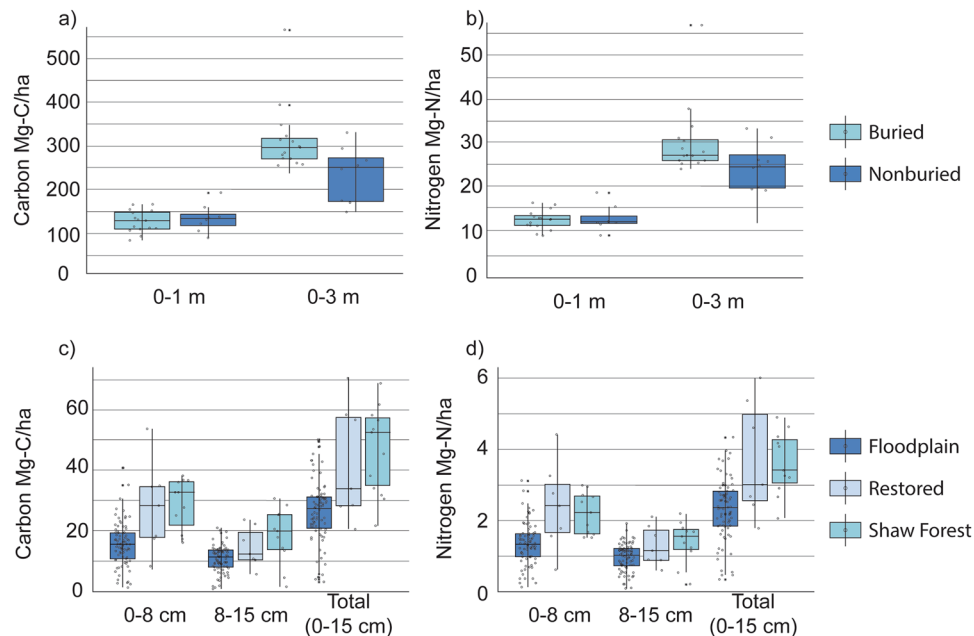
Figure 3. Box and whisker plots indicate the mean total C and N in Mg/ha for subsurface and surface samples. (a,b) Represent mean sums from 0–1 m and 0–3 m for subsurface soils with a buried horizon and subsurface soils without a buried horizon. (c,d) Represent mean sums from 0–8 cm, 8–15 cm and 0–15 cm for surface soils found in the Shaw forest, the floodplain and previously restored sites. Asterisks indicate outliers, whiskers indicate max and min values, the boxes represent the 25% and 75% quantiles and the hollow points are the discrete data points used to create the box plot.
