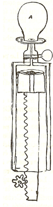
FIGURE 3. Huygens' original air pump. The receiver A is on top and the air pump with its piston is below. When the piston descends, the valve below the receiver is opened to allow the air in the receiver to expand into the cavity of the pump. When the piston ascends this valve is closed, and a second valve attached to the pump, but not shown in this diagram, is then opened to exhaust the air in the pump, ref [6] p. 313
