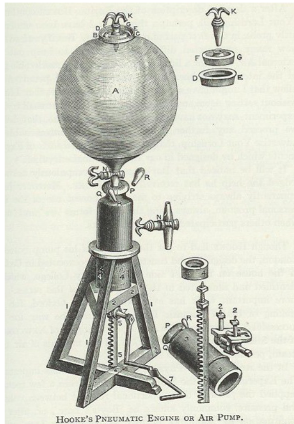
FIGURE 1. Hooke's airpump with a spherical glass receiver placed on top of it.
