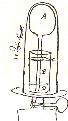
FIGURE 2. Huygens' apparatus for a Torricelli experiment placed inside the receiver of his air pump, ref. [6] p.317
