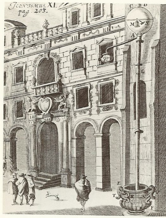
FIGURE 4. Gasparo Berti's experiment
