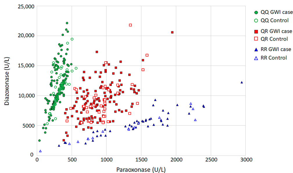
Figure 1. Plot of PON1 diazoxonase vs. paraoxonase activities for GWI cases (solid symbols) and controls (open symbols). The samples are clustered into three discrete groups based on enzyme activity, which correspond closely to QQ (green circles), QR (red squares), and RR (blue triangles) variants of the PON1 Q192R polymorphism.
