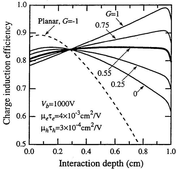
Figure 3. Calculated charge induction efficiency as a function of radiation interaction depth as measured from the full-area electrode for the coplanar-grid detector described in Fig. 2. The bias applied across the detector and the electron and hole mobility-lifetime products ( \mu_e \tau_e and \mu_h \tau_h , respectively) are listed in the figure. The charge induction efficiency is plotted for a number of values of G . For this detector and applied bias, G = 0.55 produces the most uniform response. The highly non-uniform response of a planar detector is shown for comparison.
