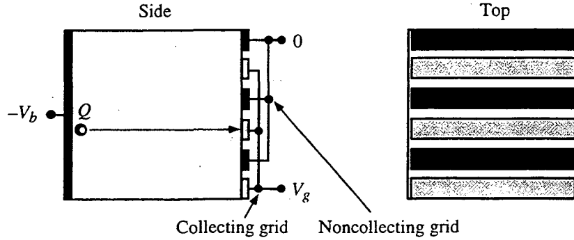
Figure 1. Schematic drawing of a coplanar-grid detector.
