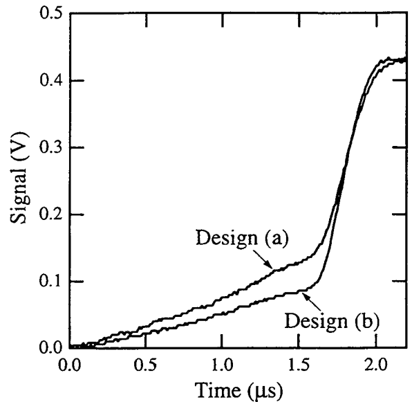
Figure 8. Measured induced charge signals on the collecting grid of a single-electrode-readout coplanar-grid detector for two different grid designs. The pulses were generated by illuminating the full-area electrode with an ^{241}\text{Am} alpha-particle source. The same CdZnTe crystal of size 9.5 \times 9.5 \times 8 \text{ mm}^3 was used for both designs and the measured mobility-lifetime products for the carriers of this crystal are \mu_e \tau_e = 4.1 \times 10^{-3} \text{ cm}^2/\text{V} and \mu_h \tau_h = 3.5 \times 10^{-4} \text{ cm}^2/\text{V} . The bias applied across the detectors was 370 V. The electrode widths and gap sizes for design (a) are w_c = 0.25 \text{ mm} , w_{nc} = 0.75 \text{ mm} , and w_g = 0.25 \text{ mm} , and those for design (b) are w_c = 0.15 \text{ mm} , w_{nc} = 0.97 \text{ mm} , and w_g = 0.18 \text{ mm} . The relative area of the design (a) collecting grid electrode is greater than that of the design (b) collecting grid electrode, therefore the charge induction during the majority of the charge collection process is greater for design (a).
