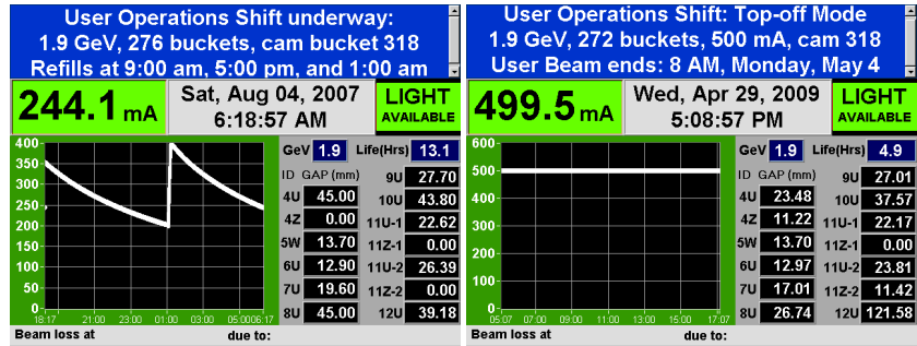
FIGURE 1. Snapshots of the 12 hour ALS status display in decaying beam operation as well as top-off. Note the difference in vertical scale (400 vs. 600 mA).
