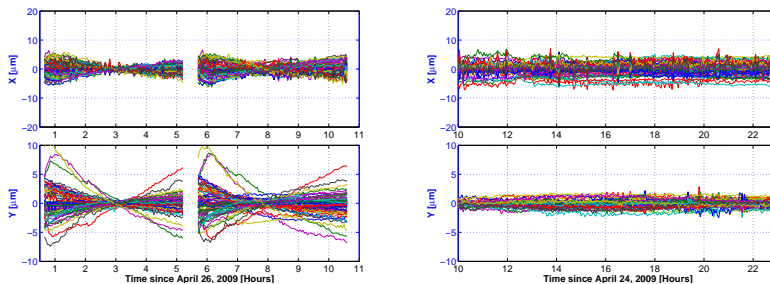
FIGURE 2. Medium term (10-20 h) orbit stability for top-off mode (right) compared to decaying beam operation (left).
